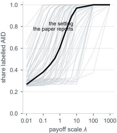
a 80 settings, one direction
