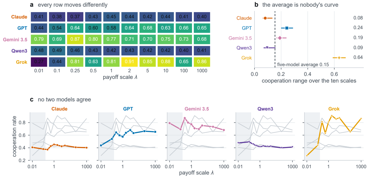
Figure 2: Cooperation rates as a function of the payoff scale across five models. (a) Model-by-scale cooperation matrix: mean cooperation for each of the five models at each of the ten payoff scales \lambda \in [0.01, 1000] , with the value shown in each box. (b) Within-model cooperation range (maximum minus minimum rate across the ten scales) compared against the pooled five-model range (0.154, vertical dashed line). Confidence intervals are 95% percentile intervals from 1,500 whole-dyad bootstrap resamples. (c) Small multiples per model: the focal model is drawn with its designated colour and marker, with the other four models shown behind in grey for context. Shaded bands mark the sub-unit regime ( \lambda \leq 0.1 ). Each model-by-scale cell pools 200 dyads (400 agent-games), 20,000 agent-games in all.
