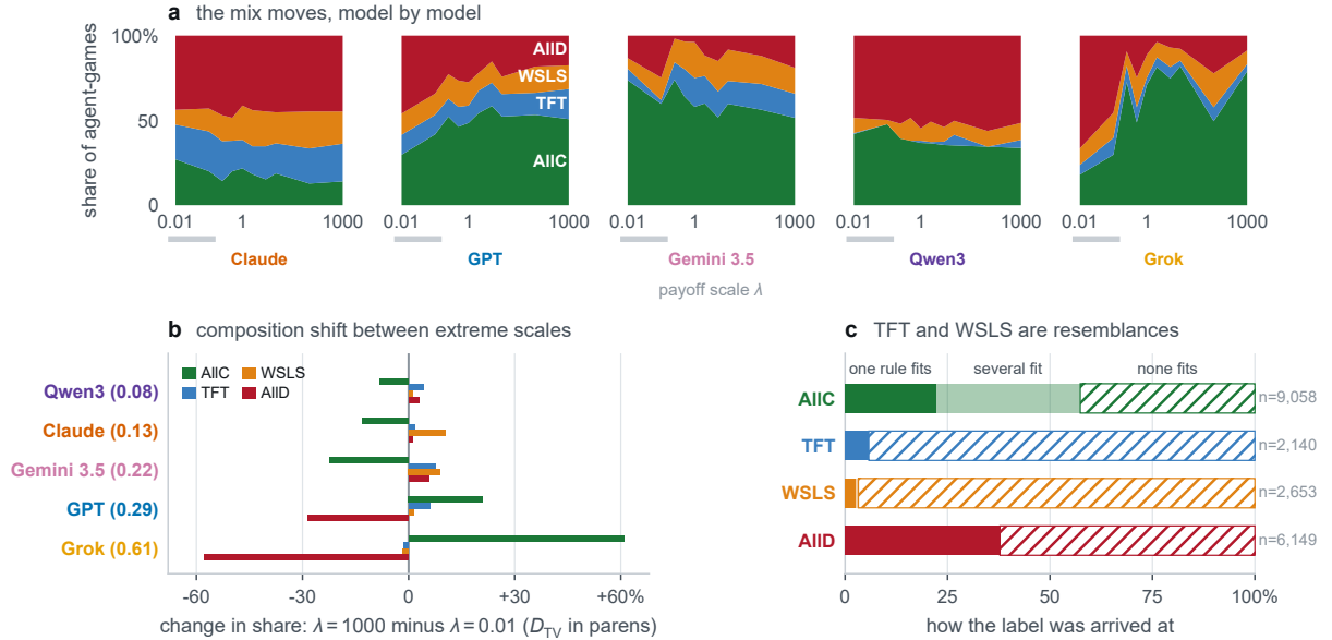
Figure 5: Strategy attribution across payoff scales, composition shift, and provenance breakdown. (a) Stacked area share of canonical memory-one strategy attributions (AIIC, AIID, TFT, WSLs) across the ten payoff scales for each of the five models. (b) Net strategy share changes between extreme scales ( \lambda = 10^3 minus \lambda = 0.01 ) across the four canonical rules with total variation distance D_{TV} in parentheses. (c) Strategy read-out provenance: exactly deduced (single canonical match), ambiguous (multiple matching rules), and unmatched (LSTM attribution on trajectories consistent with no standard rule). Over the corpus, 94.6% of Tit-for-Tat and 97.1% of Win-Stay-Lose-Shift labels are attributions on unmatched play, establishing that labels indicate resemblance rather than faithful execution.
