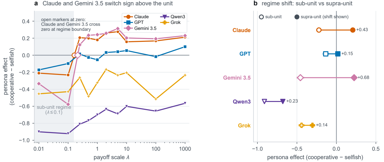
Figure 4: Persona effect and sub-unit inversion against the payoff scale. The persona effect is the cooperation rate under the cooperative persona minus that under the selfish persona. (a) Difference in cooperation rate across scales \lambda , with the sub-unit regime ( \lambda \leq 0.1 ) shaded where all five models cooperate more under the selfish prompt. (b) Regime means comparing sub-unit ( \lambda \leq 0.1 , open circles) with supra-unit ( \lambda \geq 0.25 , filled circles) regimes (table 2).
