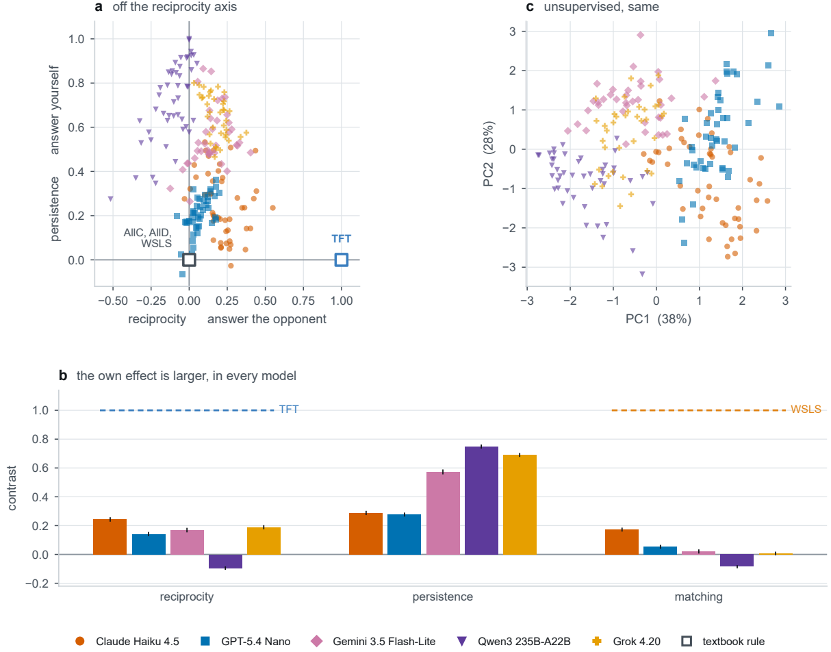
Figure 7: Own-action conditioning exceeds partner-action conditioning at the model level.
