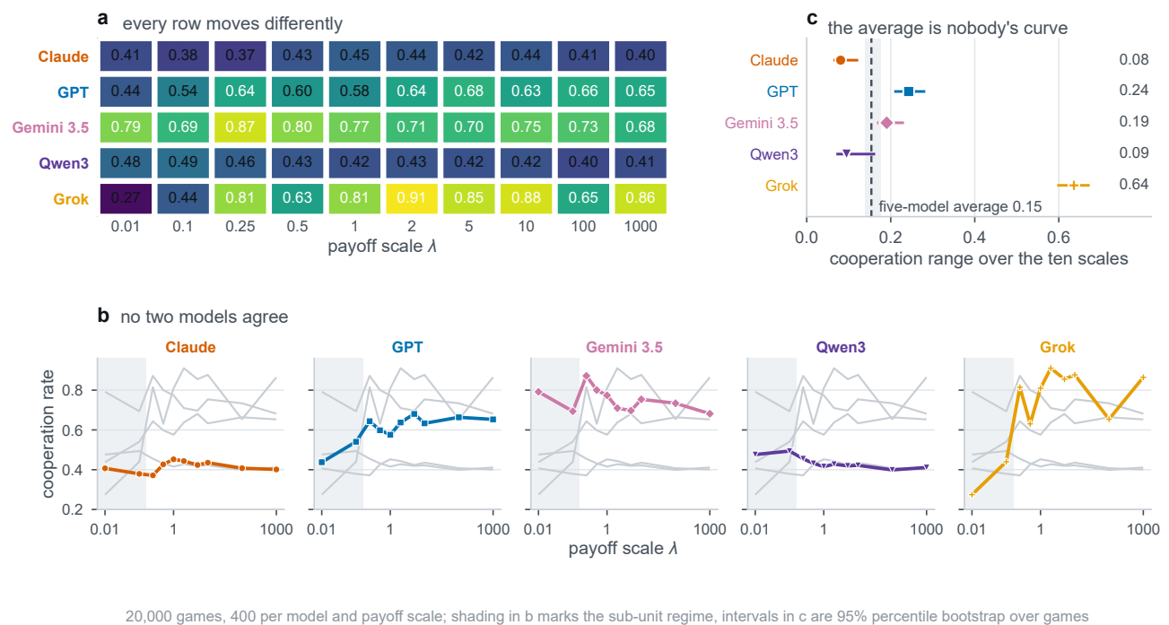
Figure 2. Cooperation against the payoff scale across five frontier models. (a) Model-by-scale cooperation matrix: mean cooperation for each of the five models at each of the ten payoff scales \lambda \in [0.01, 1000] , with the value printed in each tile. (b) Small multiples per model: the focal model is drawn with its designated colour and marker, with the other four models shown behind in grey for context. Shaded bands mark the sub-unit regime ( \lambda \leq 0.1 ). (c) Within-model cooperation range (maximum minus minimum rate across the ten scales) compared against the pooled five-model range (0.154, vertical dashed line). Confidence intervals are 95% percentile intervals from 1,500 whole-dyad bootstrap resamples.
