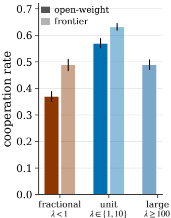
a by notation regime
