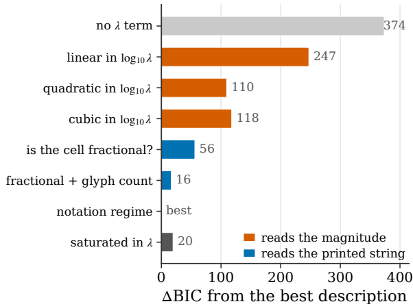
b what the response tracks
