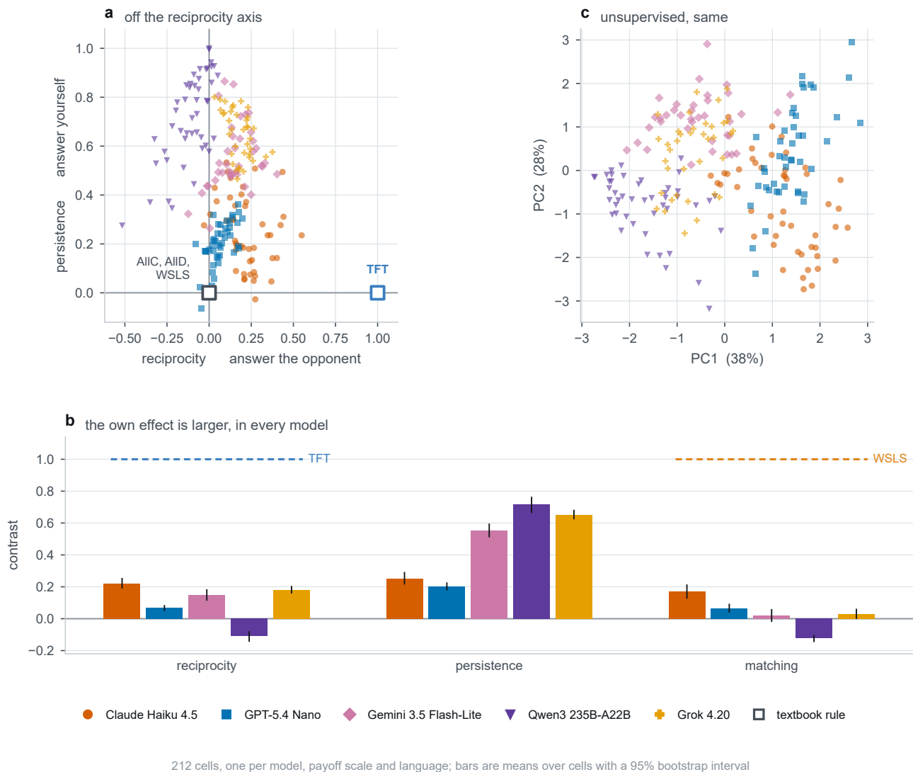
Figure 8. The agents condition on themselves, not on their partner. (a) Cells in the reciprocity by persistence plane, with the canonical rules at their exact coordinates; AIIC, AIID and win-stay lose-shift all have both main effects zero and so coincide at the origin. (b) The three contrasts per model, against the value each canonical rule would give, with 95% bootstrap intervals over cells. (c) The first two principal components of the raw five-vector, which is given no knowledge of the contrasts and recovers the same geometry. A cell is one model, payoff scale and prompt language; a predecessor observed fewer than thirty times yields no estimate and the cell is dropped, leaving 212 of 250.
