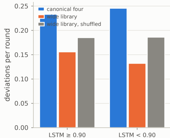
a A wider vocabulary closes the gap
