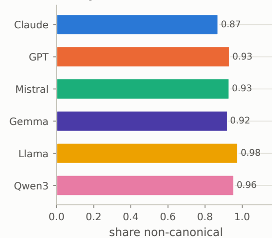
f Every model, most of the time
