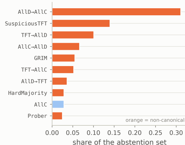
c Nearest rule, wide library
