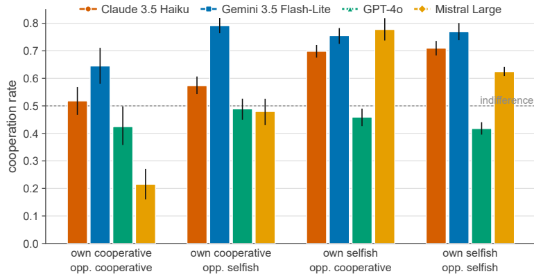
Cooperation by persona pairing
