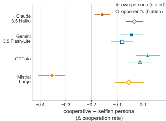
Steerability, 95% CI
