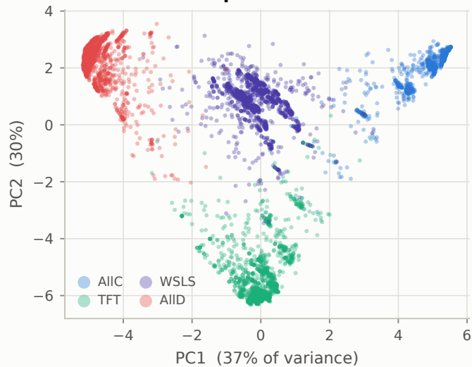
Hidden state separates the rules
