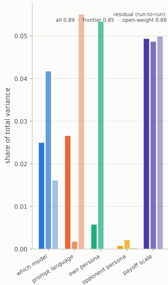
Variance decomposition bar triplet = all runs · frontier · open-weight
