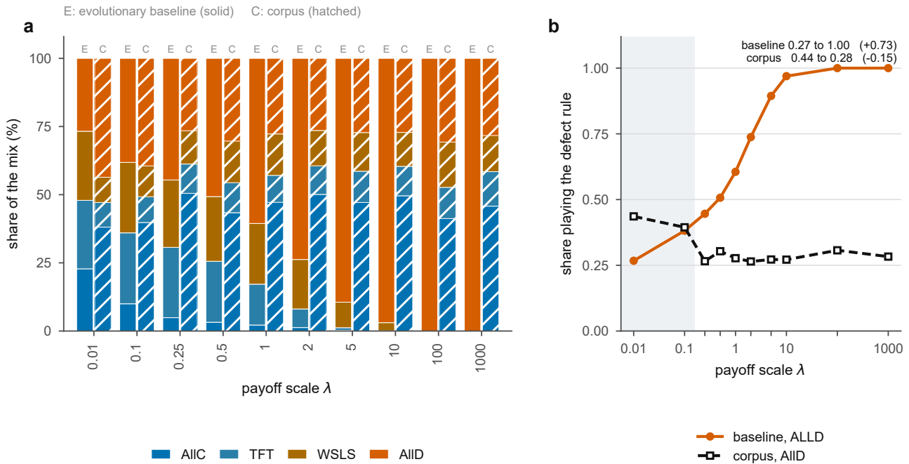
Figure C.1. The evolutionary baseline against the corpus, at matched payoff scales. (a) Stationary frequency of each canonical strategy under the small-mutation limit ( Z = 100 , \beta = 0.1 , r = 10 , \varepsilon = 0.05 ), beside the pooled label composition of the five main-text models at the same payoff scale. (b) The share playing Always Defect alone, the one series on which the two disagree in sign: across the ten scales the baseline rises from 0.27 to 1.00 while the corpus falls from 0.44 to 0.28.
