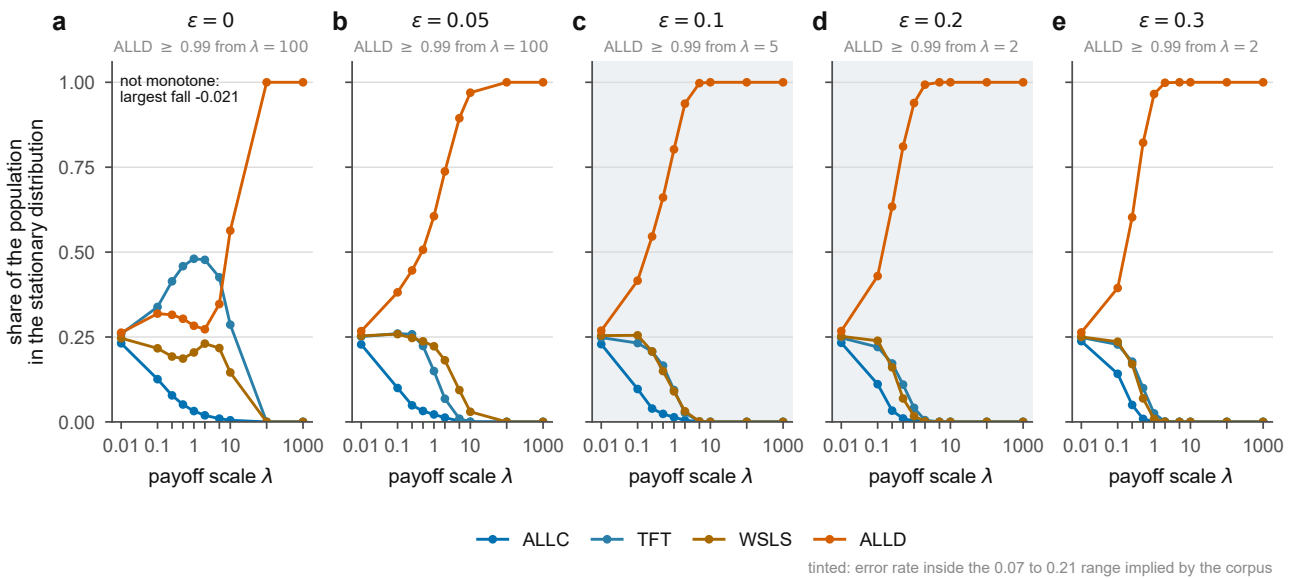
Figure C.2. The evolutionary baseline across the payoff grid and the execution-noise levels. Stationary frequency of each of the four canonical strategies against the payoff scale, one panel per execution-error rate \varepsilon . Always Defect rises with \lambda at every level, and does so sooner the noisier execution is; the rise is monotone at every positive \varepsilon and dips slightly before rising in the error-free corner \varepsilon = 0 (table C.2).
