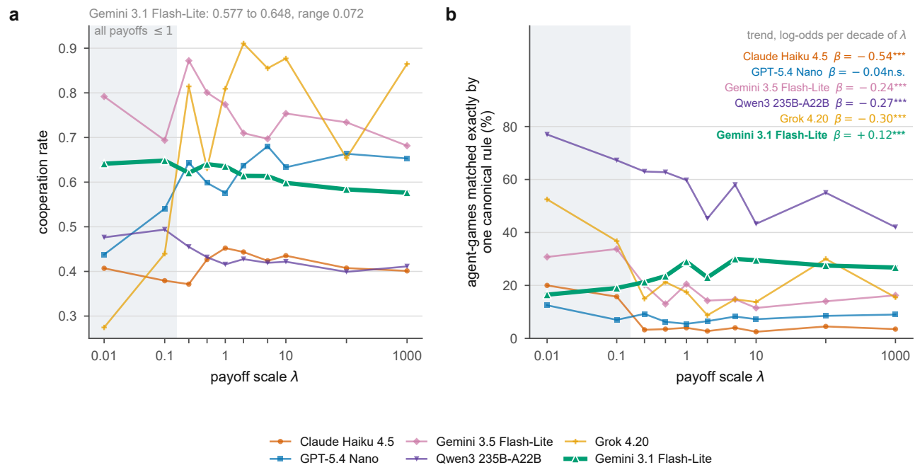
Figure B.1. The sixth model beside the five reported in the main text. Gemini 3.1 Flash-Lite is drawn heavier and in front. (a) Cooperation against the payoff scale, where it sits inside the spread of the other five. (b) Share of agent-games matched exactly by one canonical rule, with each model's trend per decade of \lambda . It is the only model of the six whose trend is positive.
