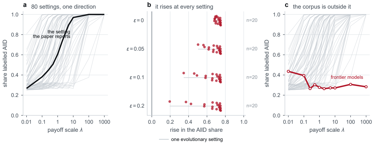
80 settings: Z \in \{50, 100, 200, 500\} , \beta \in \{0.01, 0.05, 0.1, 0.5, 1\} , \epsilon \in \{0, 0.05, 0.1, 0.2\} , ten payoff scales, each solved at 200 digits. The rise is monotone at every positive \epsilon ; the exceptions are at \epsilon = 0 , where the share dips before it rises
