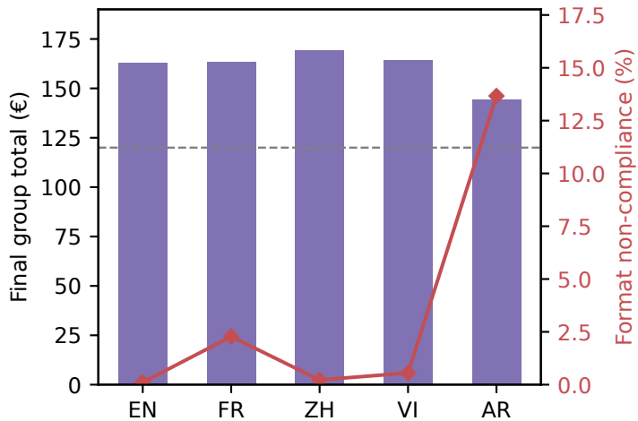
(b) Language — Gemma-2-9B
