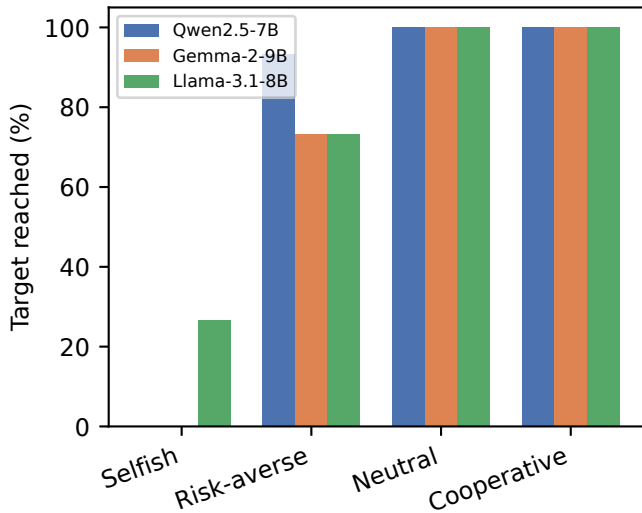
(a) Disposition prompt
