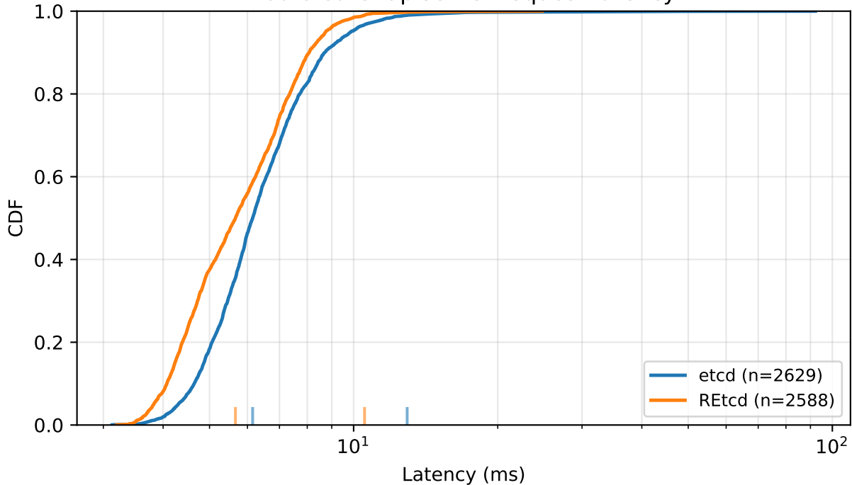
Pod create: apiserver request latency
