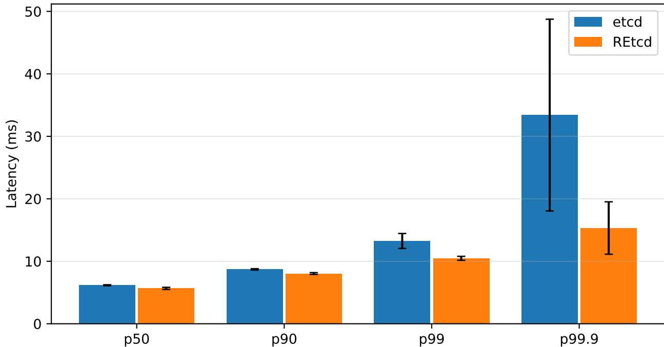
Pod create: latency percentiles (mean \pm std across trials)
