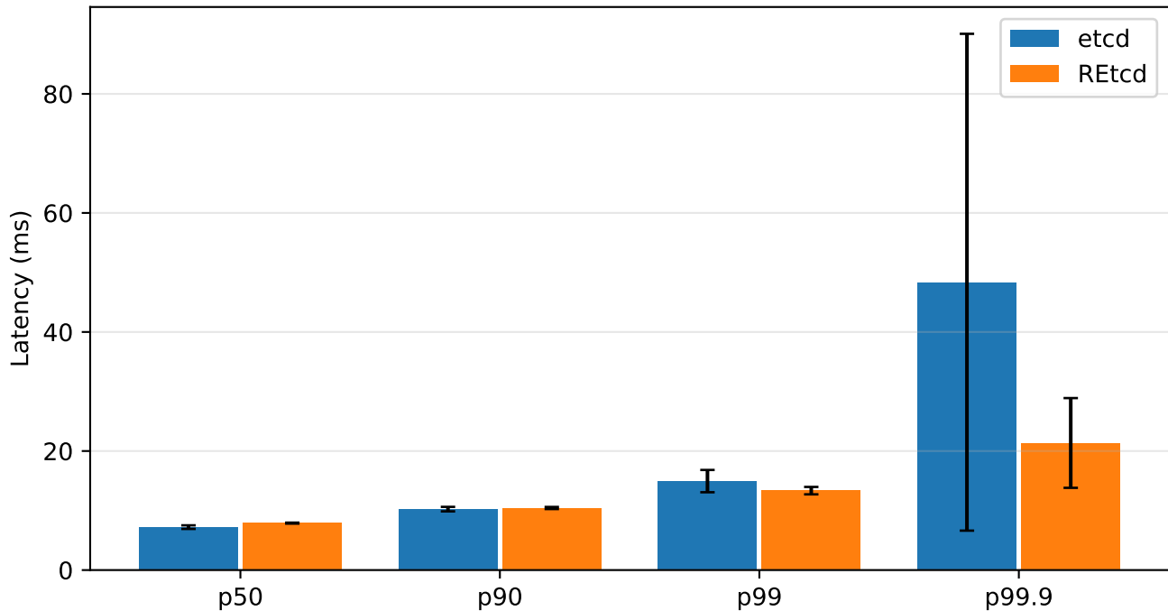
Pod delete: latency percentiles (mean \pm std across trials)
