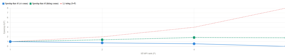
Figure 6 – Plot on Speedup Analysis (communication time and computing time) with 4 scenarios (P increase, Threads decrease)
