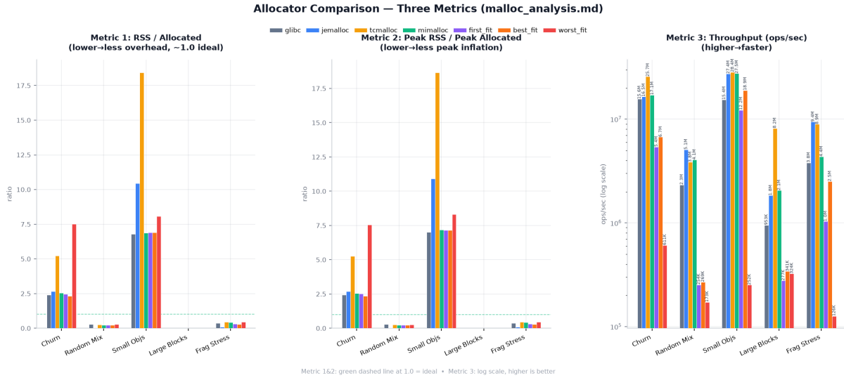
Figure 2: Phase 2: Three-metric cross-allocator comparison. Metric 1 and 2: green dashed line at 1.0 = ideal. Metric 3: log scale, higher is better.
