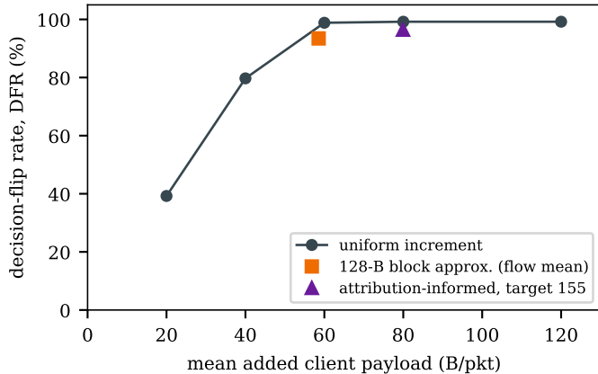
(a) Model-B, same 4,799 base flows
