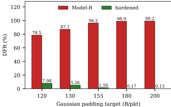
(b) Before and after hardening
