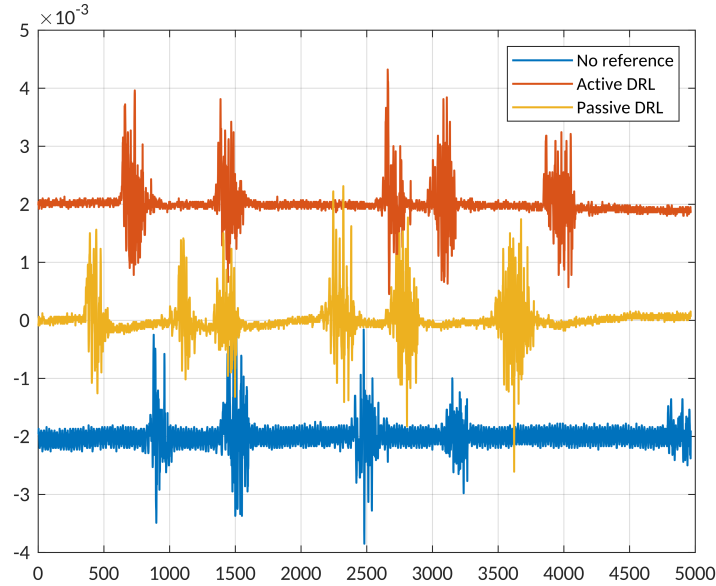
Figure 3.3. Measured differential EMG with no reference (blue), passive referencing to ground (yellow), active DRL (red)
