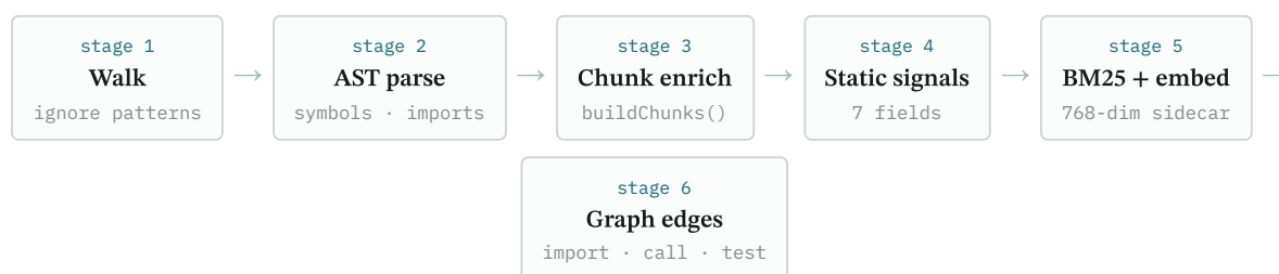
Figure §5.2. Six-stage index build pipeline.
