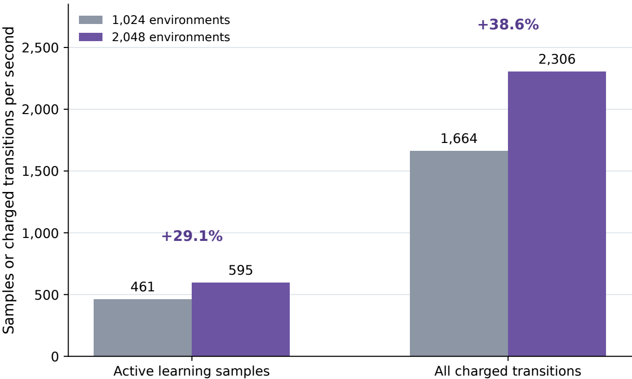
B Training capacity, including startup
