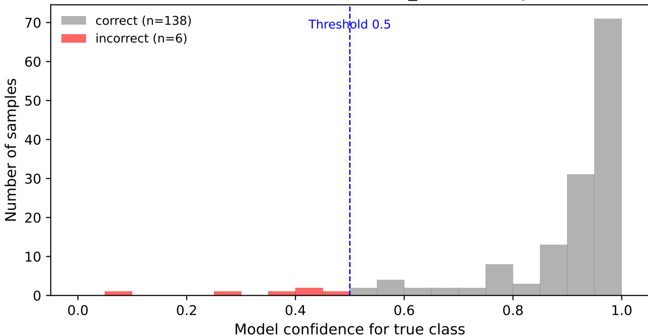
Confidence distribution - efficientnet_b1 (Accuracy = 0.958)
