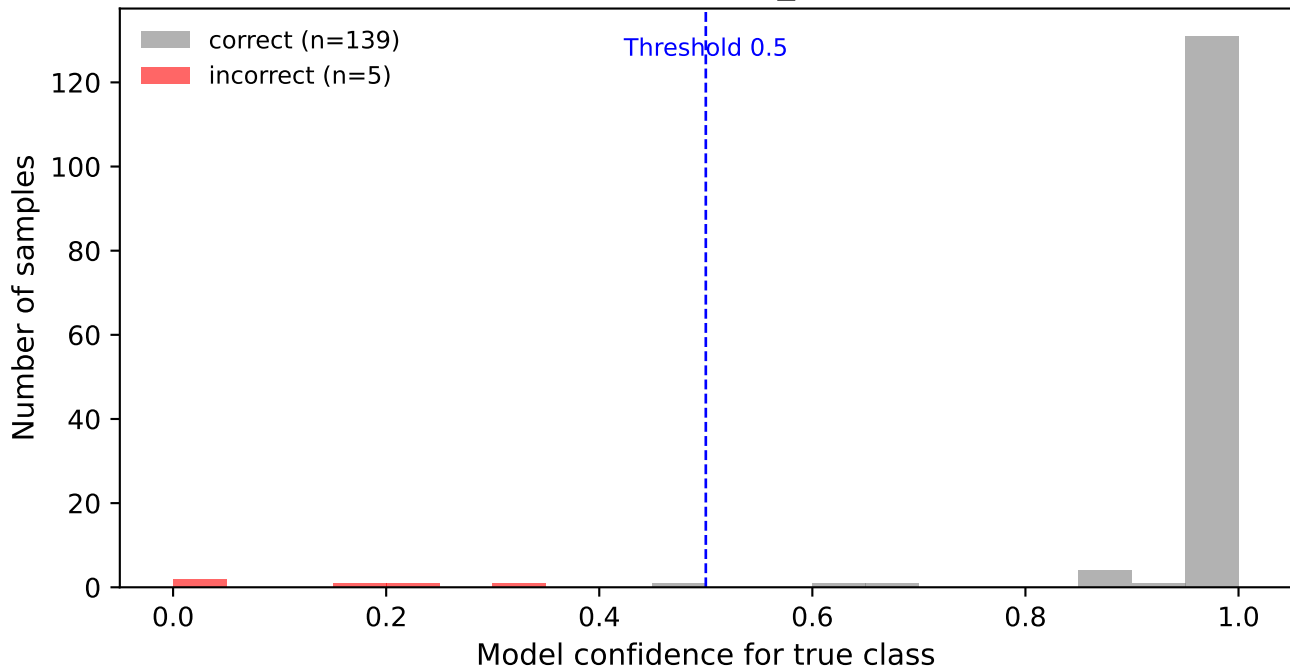
Confidence distribution - vgg16_bn (Accuracy = 0.965)
