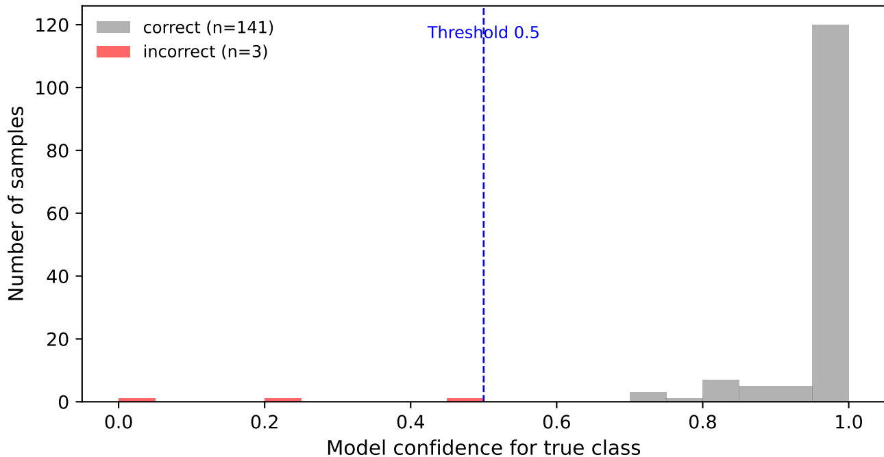
Confidence distribution - resnet18 (Accuracy = 0.979)
