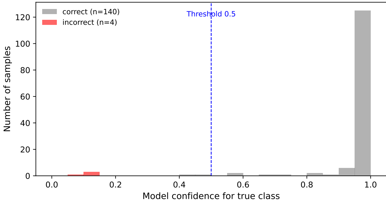
Confidence distribution - resnet101 (Accuracy = 0.972)
