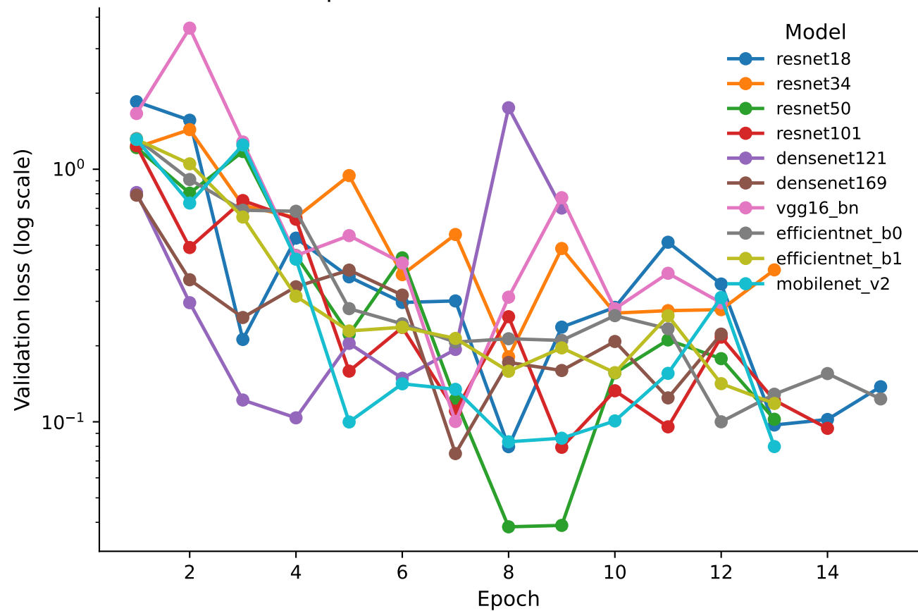
Comparison of models - validation loss
