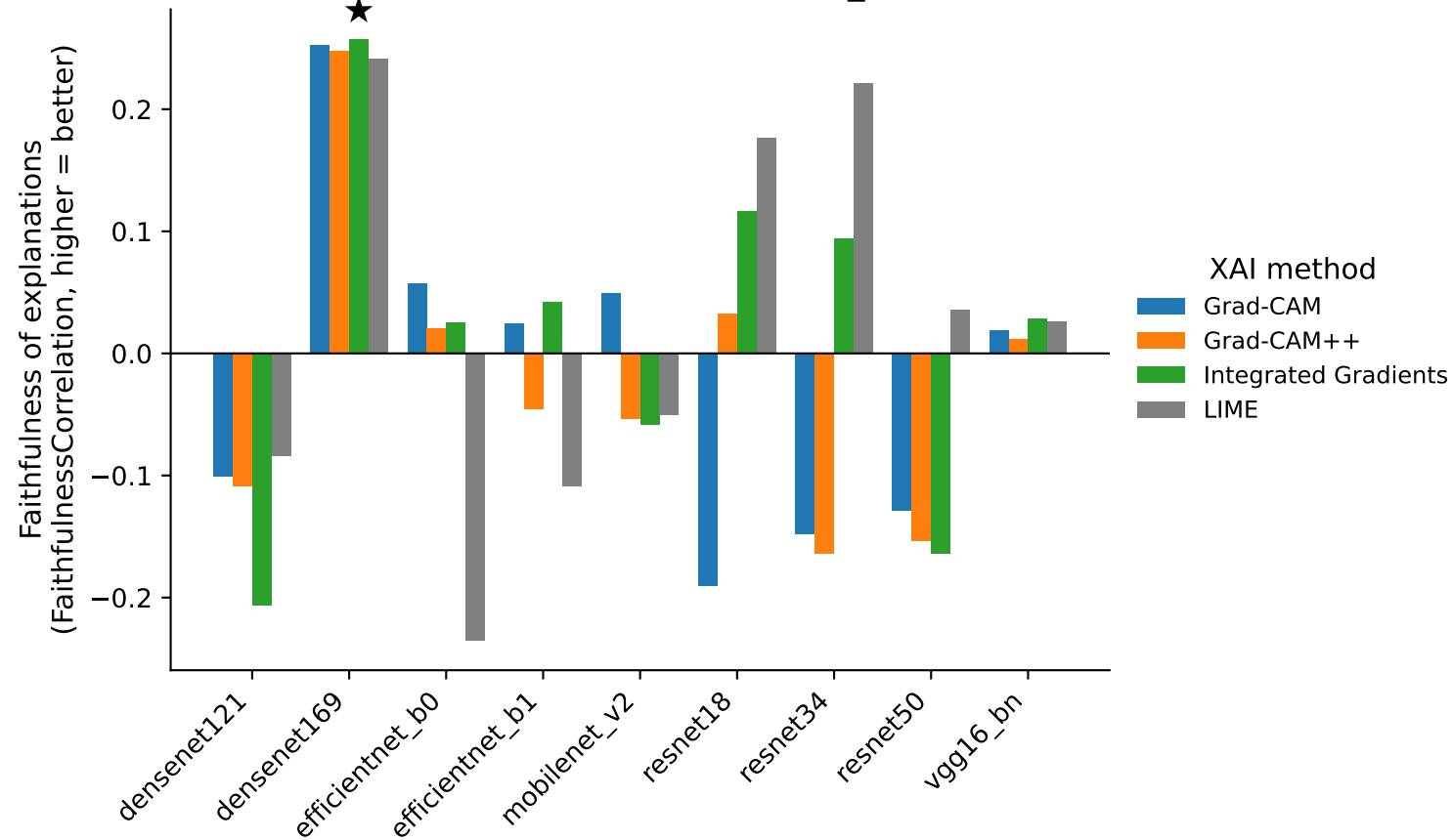
★ Quantus metric - faithfulness_corr
