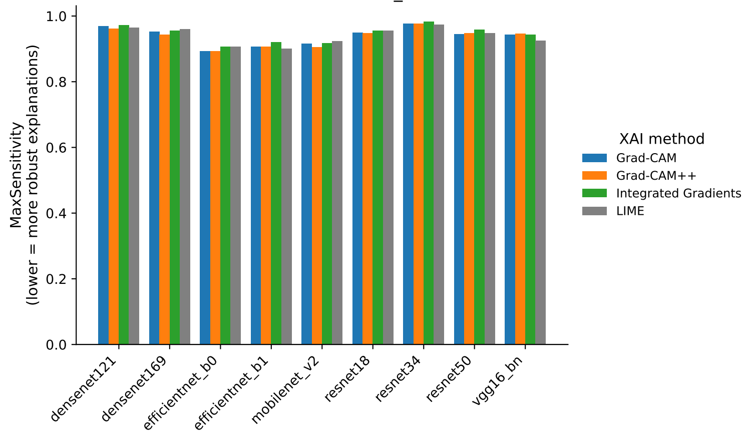
Quantus metric - max_sens
