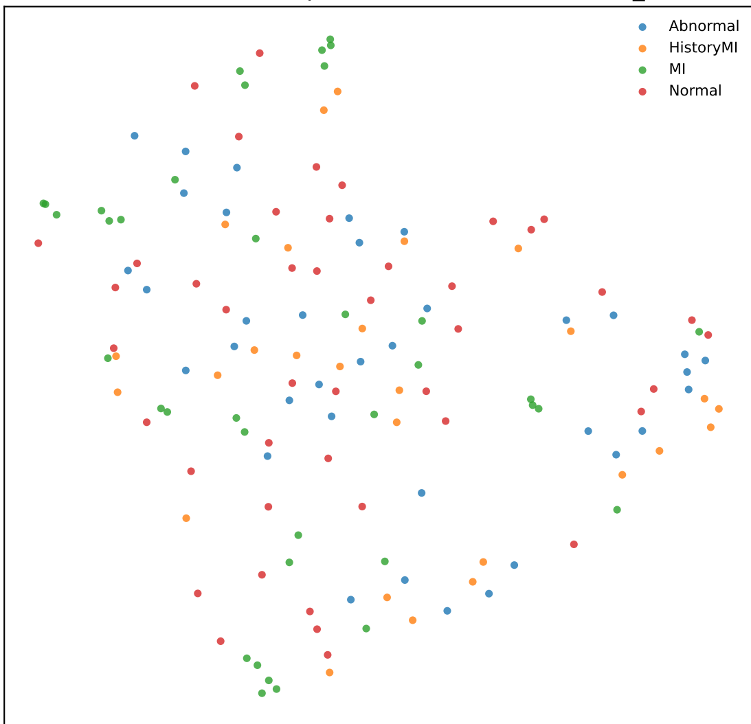
UMAP of feature representations - efficientnet_b0
