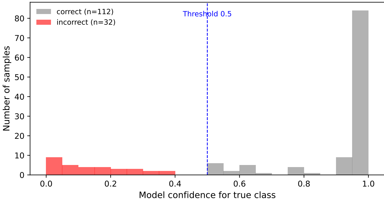
Confidence distribution - resnet101 (Accuracy = 0.778)
