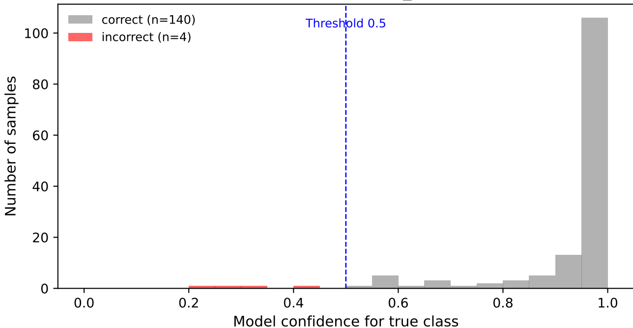
Confidence distribution - efficientnet_b1 (Accuracy = 0.972)
