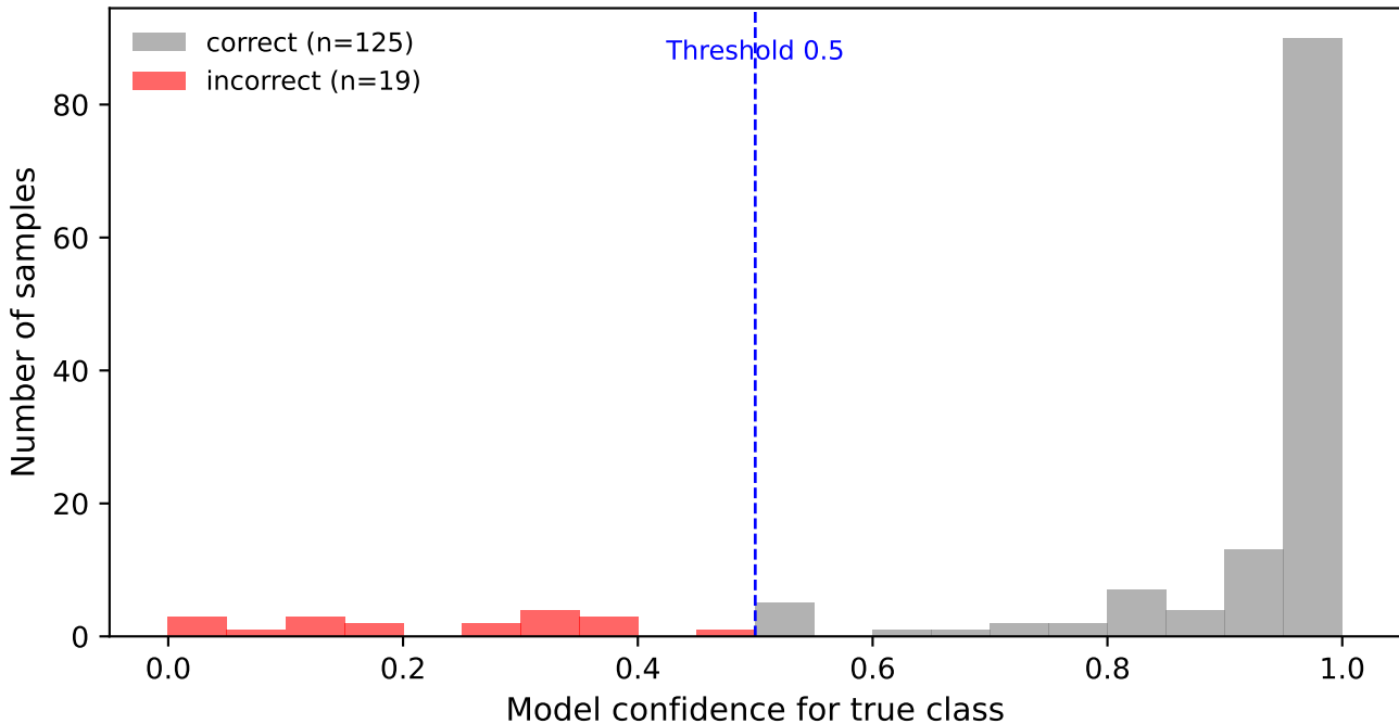
Confidence distribution - densenet169 (Accuracy = 0.868)
