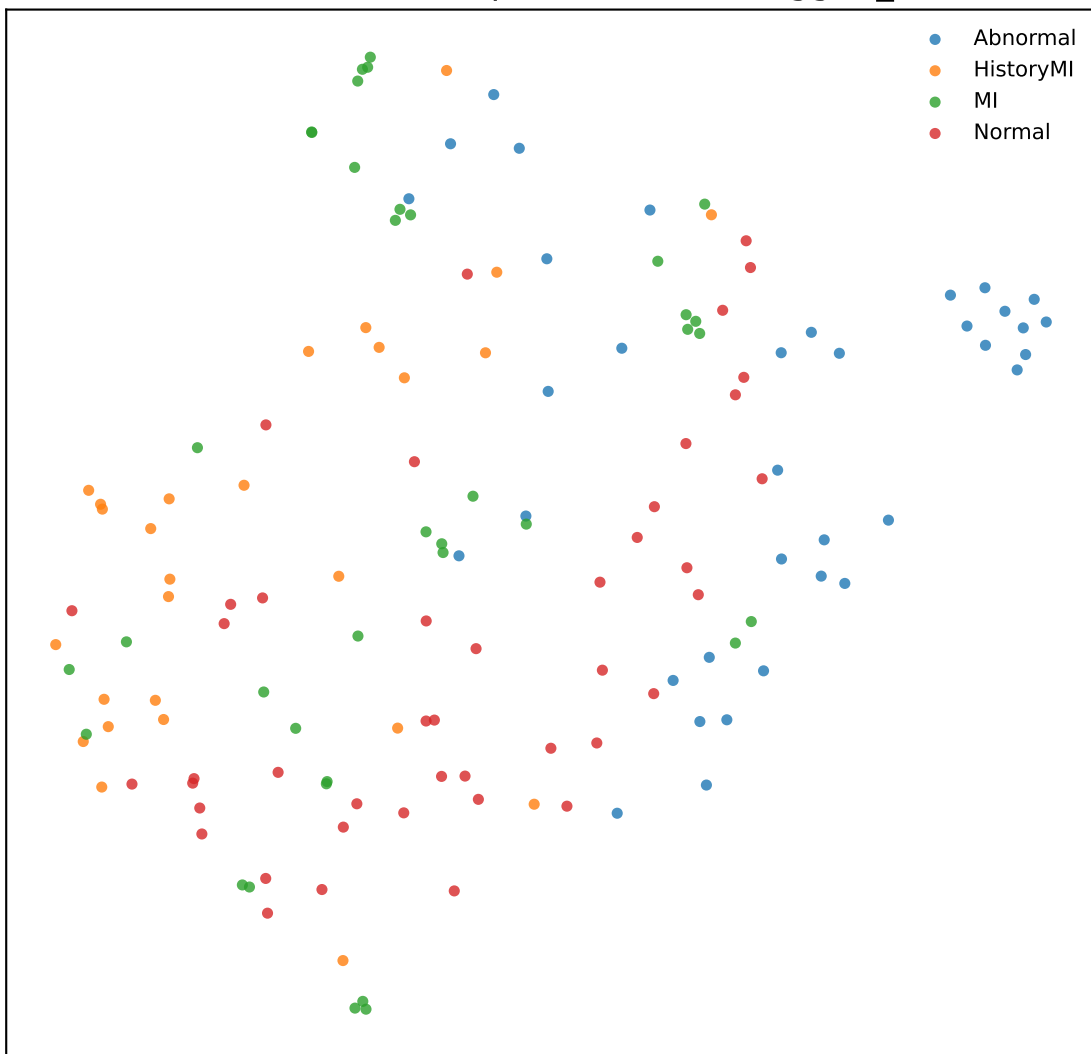
UMAP of feature representations - vgg16_bn
