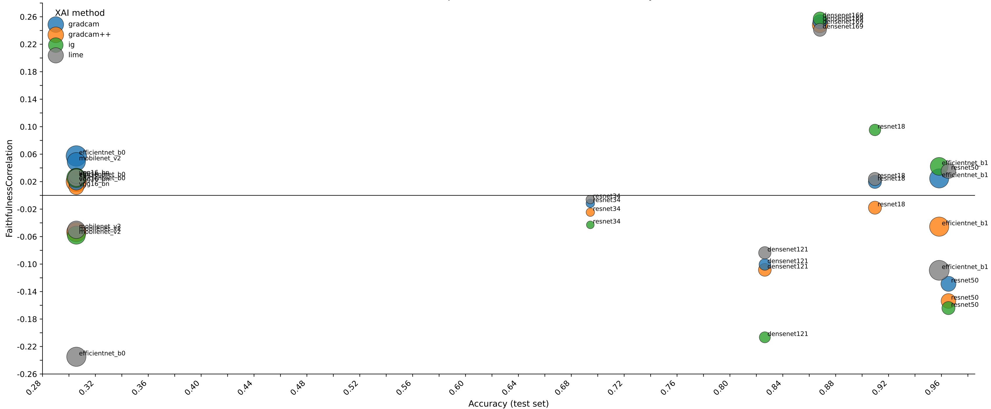
Trade-off: model performance vs. explanation quality (Bubble size \approx explanation robustness, 1 - \text{MaxSensitivity} )
