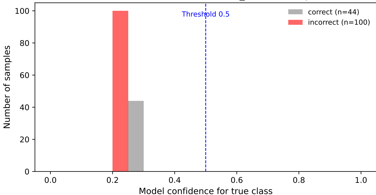
Confidence distribution - efficientnet_b0 (Accuracy = 0.306)
