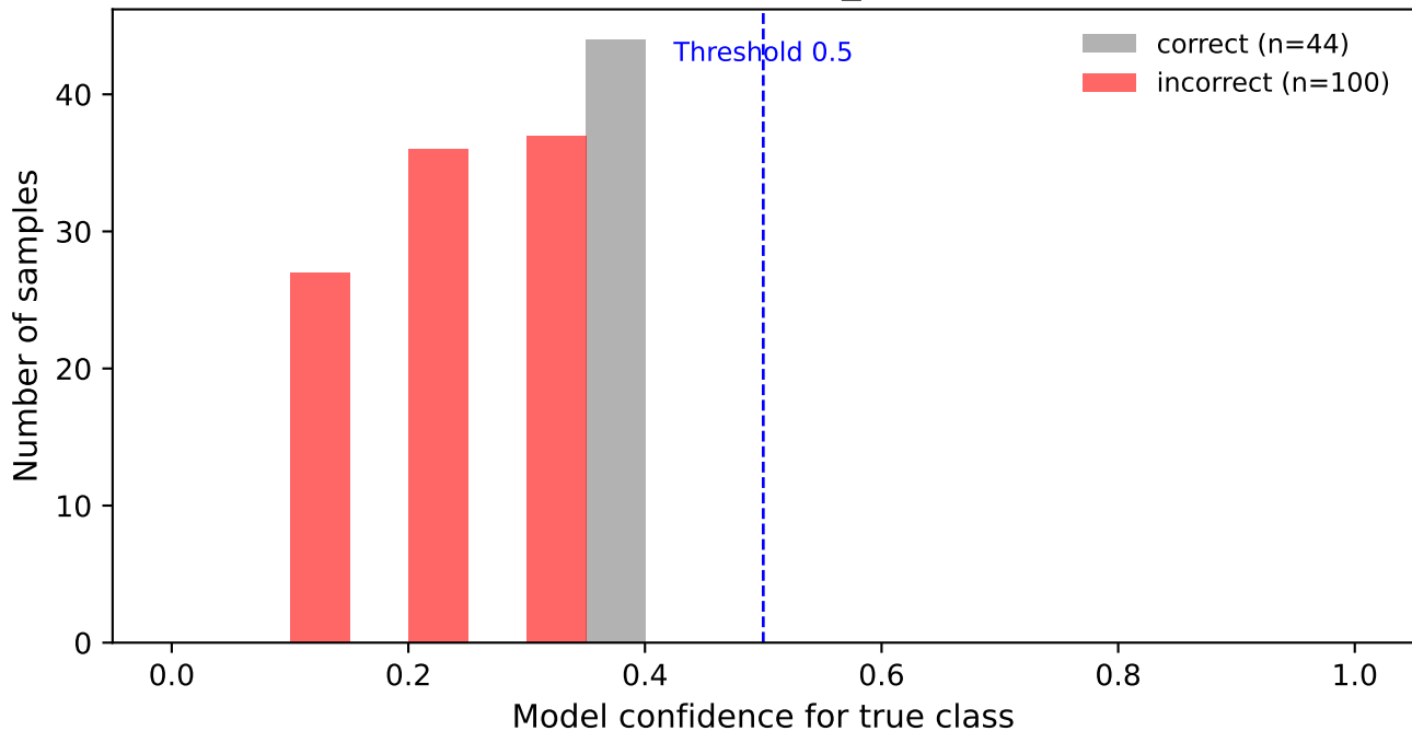
Confidence distribution - vgg16_bn (Accuracy = 0.306)
