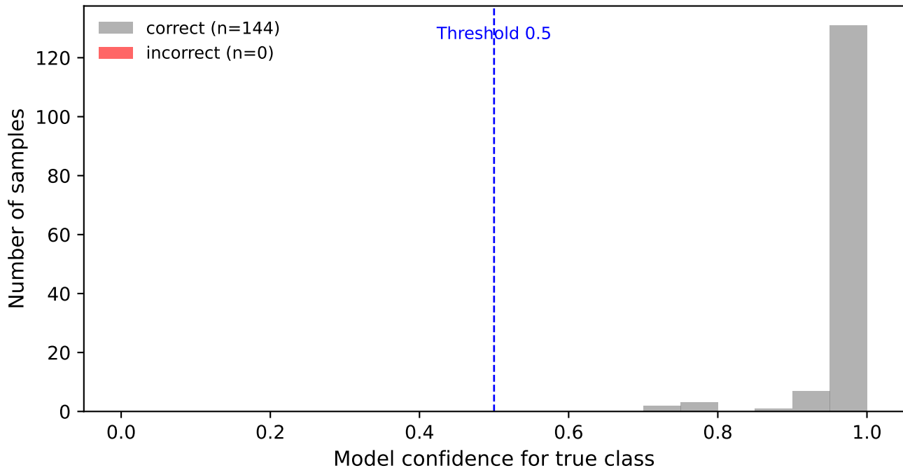
Confidence distribution - resnet50 (Accuracy = 1.000)
