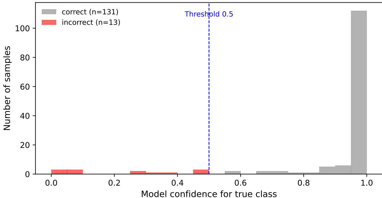
Confidence distribution - resnet18 (Accuracy = 0.910)
