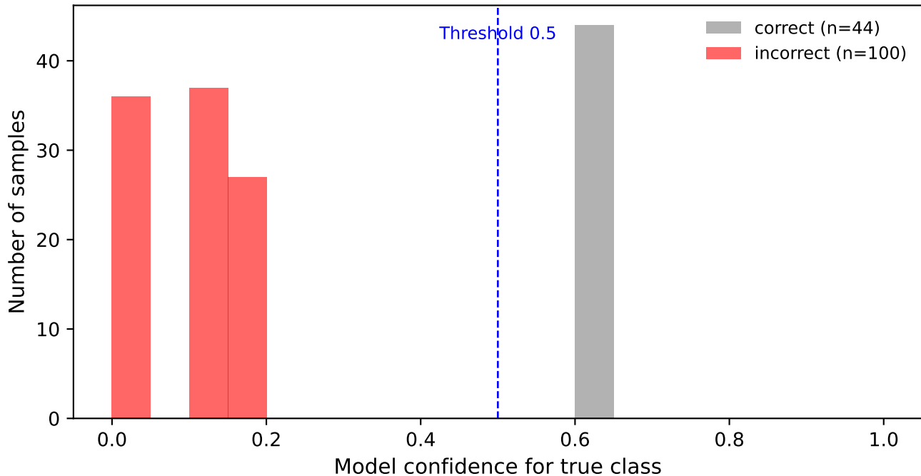
Confidence distribution - mobilenet_v2 (Accuracy = 0.306)
