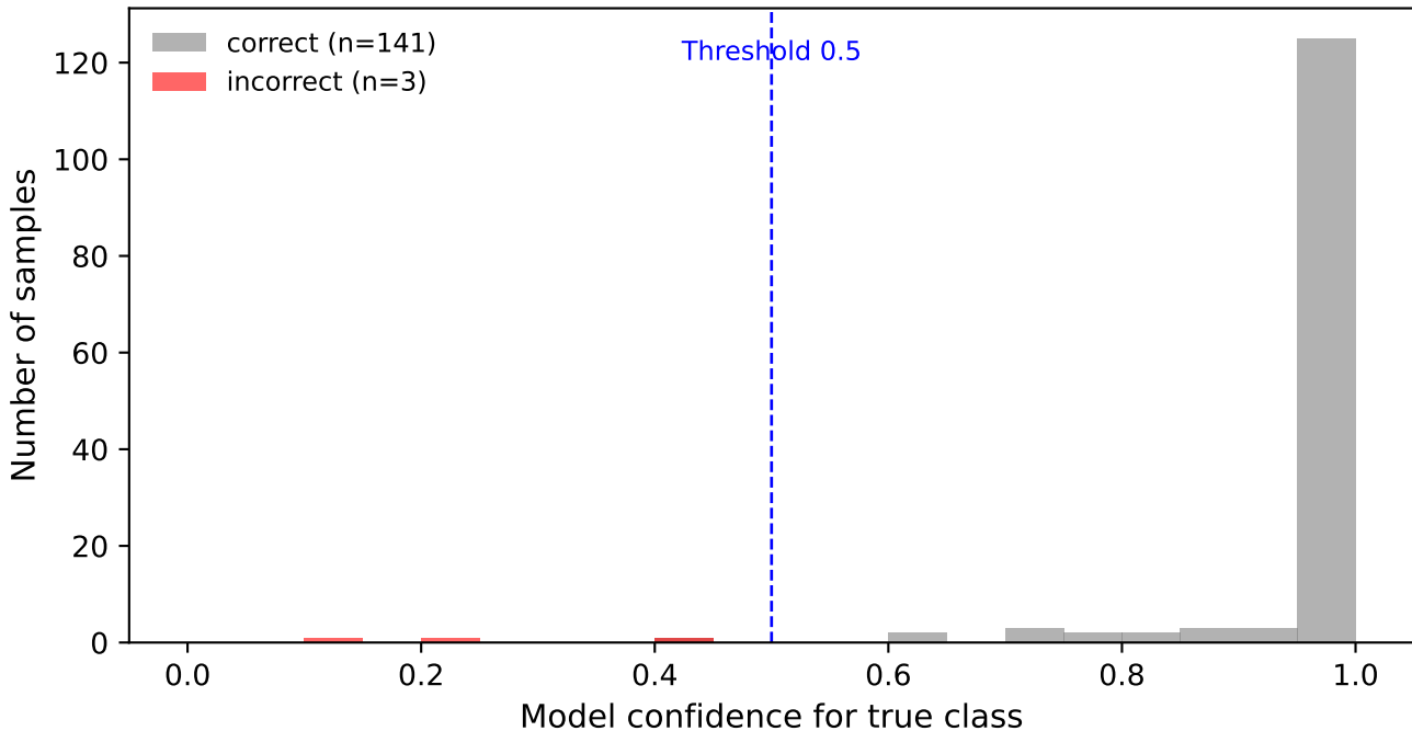
Confidence distribution - densenet169 (Accuracy = 0.979)
