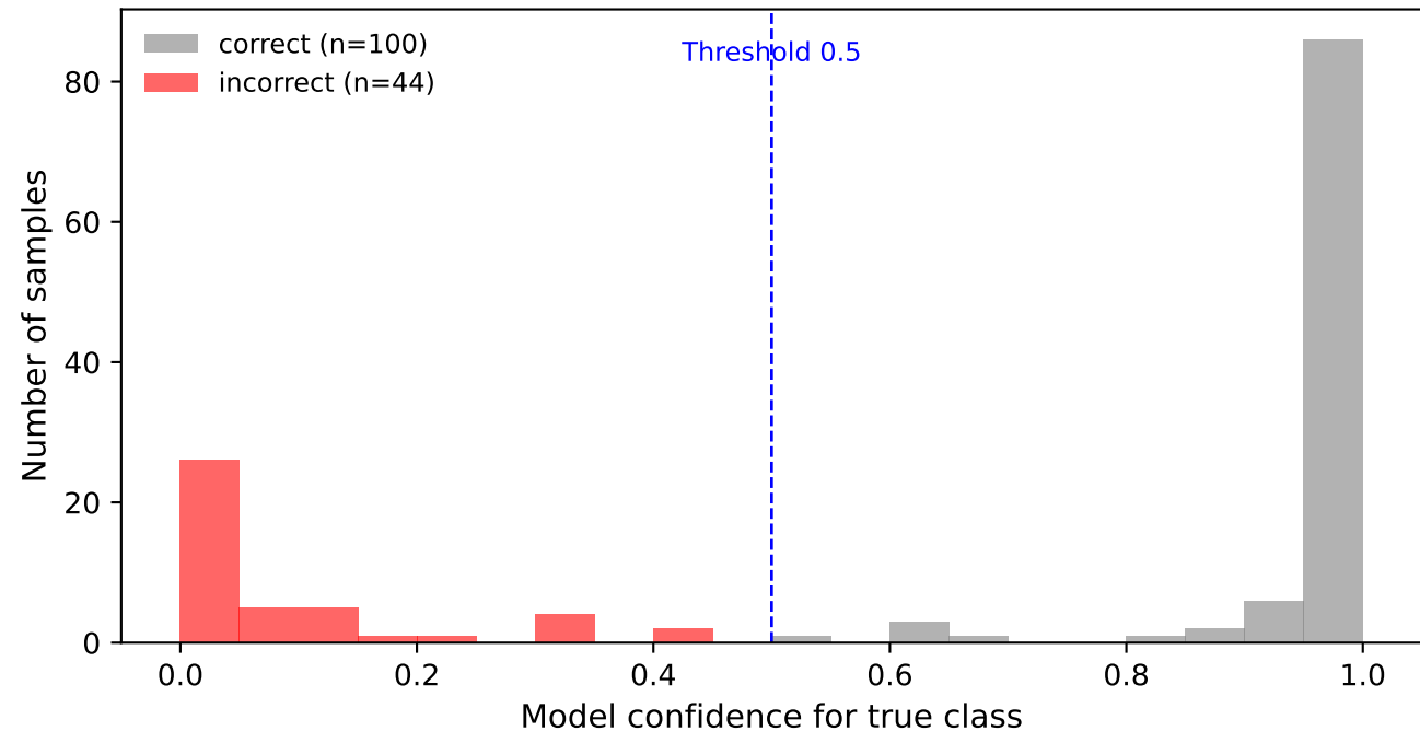
Confidence distribution - resnet34 (Accuracy = 0.694)
