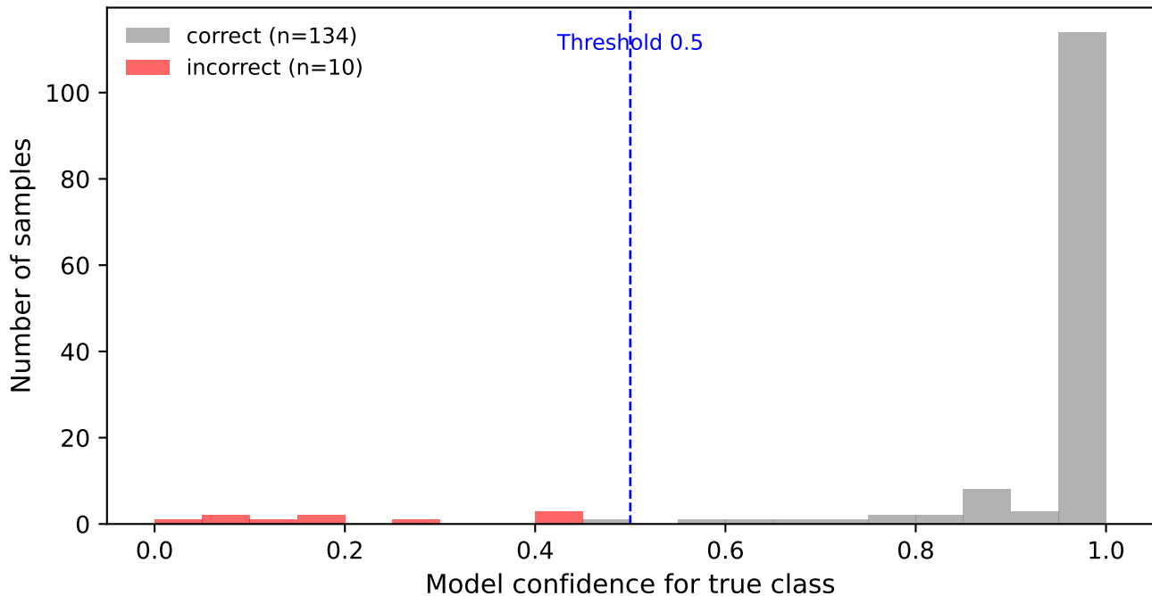
Confidence distribution - resnet34 (Accuracy = 0.931)
