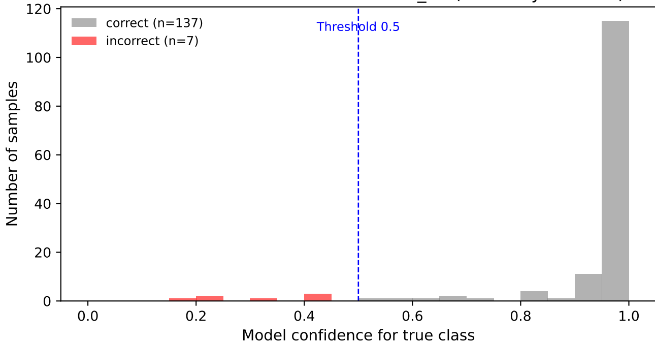
Confidence distribution - efficientnet_b0 (Accuracy = 0.951)
