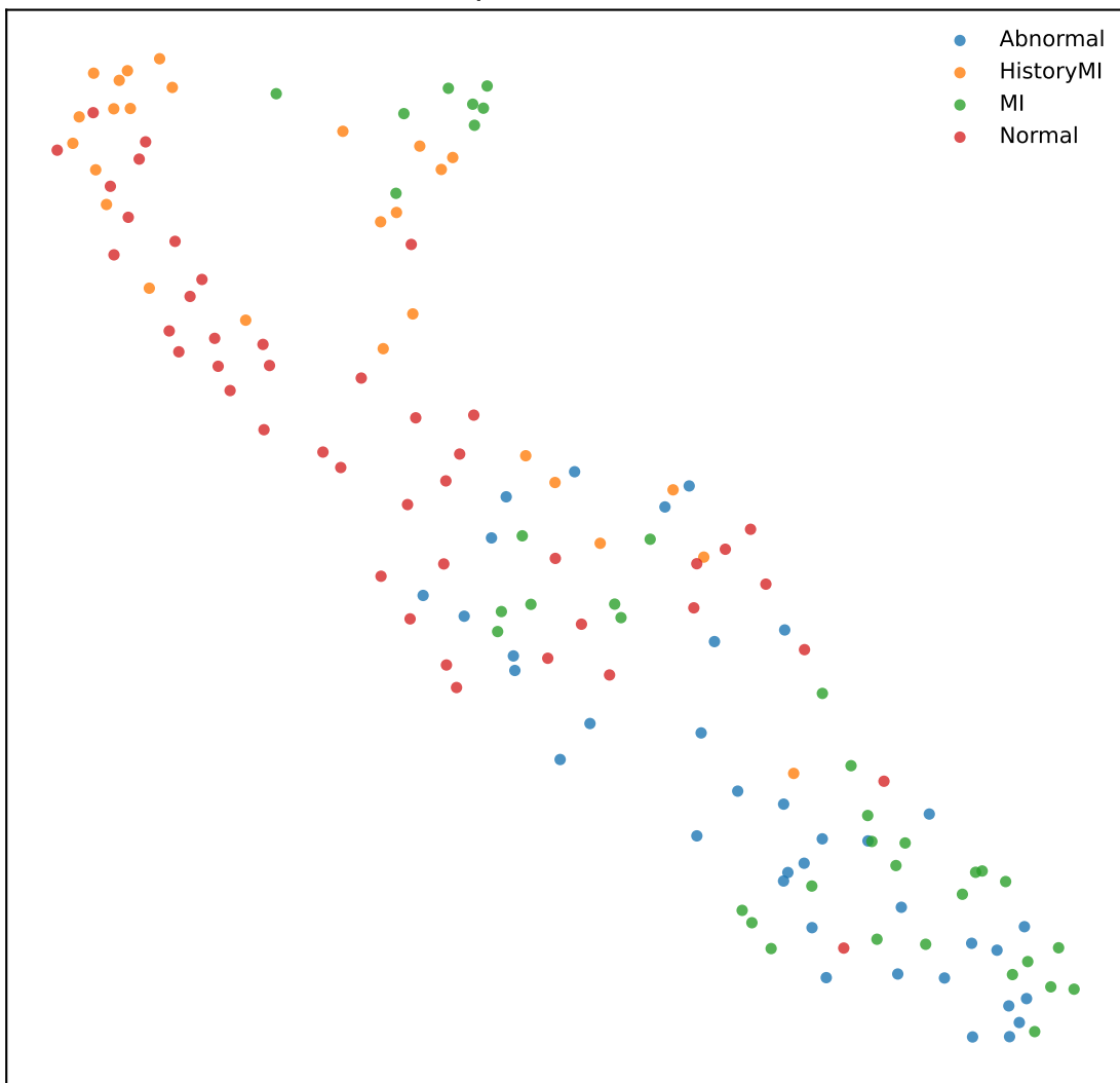
UMAP of feature representations – densenet169
