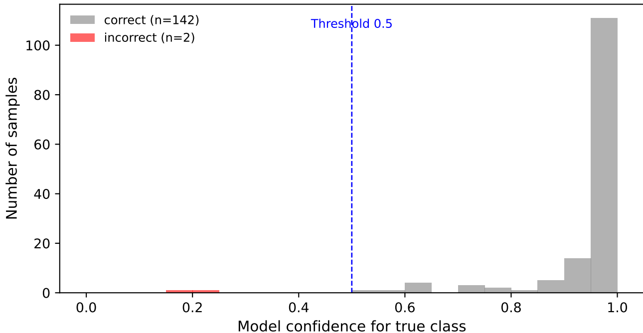
Confidence distribution - densenet121 (Accuracy = 0.986)
