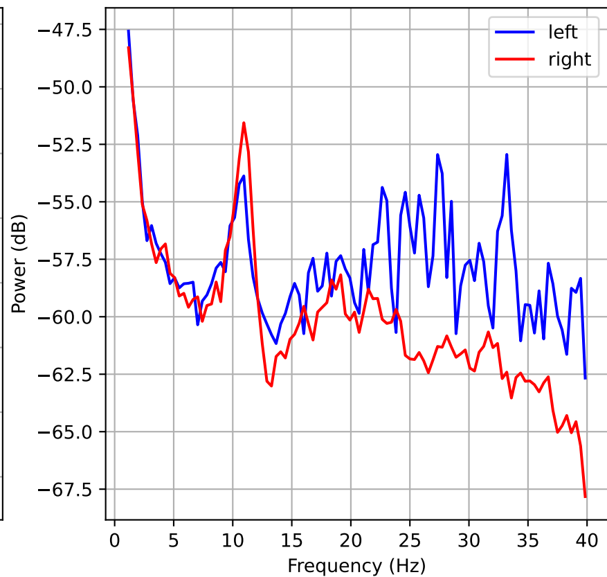
PSD - Channel C4
