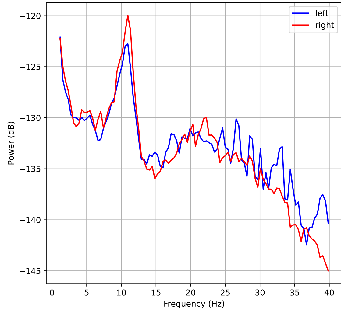
PSD - Channel C4 lap
