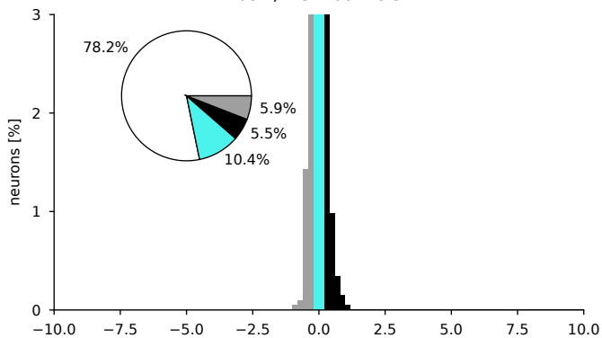
calcium, first 100 trials
