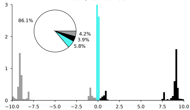
calcium2, last 100 trials
