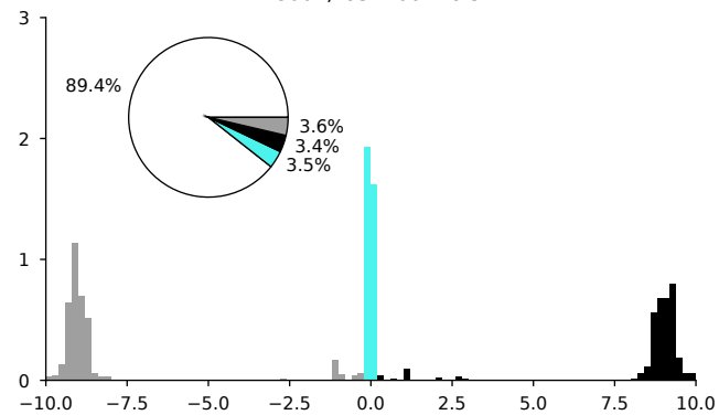
bcm2, last 100 trials
