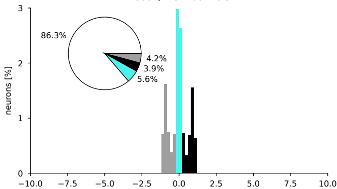
bcm2, first 100 trials
