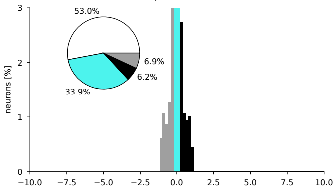
calcium2, first 100 trials
