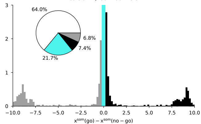
calcium2, last 100 trials
