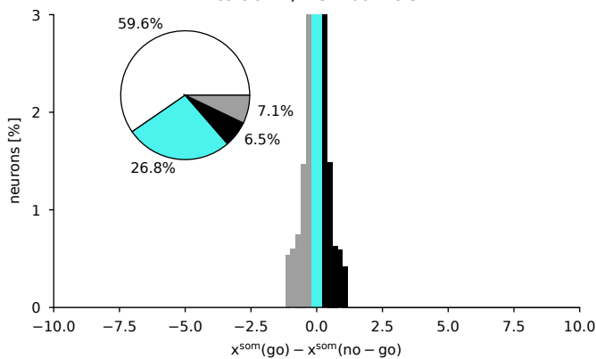
calcium2, first 100 trials
