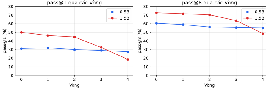
Fig. 1. Design P: pass@1 and pass@8 across five rounds for both model sizes. Both metrics fall for both models. Section 4.3 shows that this pattern does not survive isolation and held-out evaluation.
