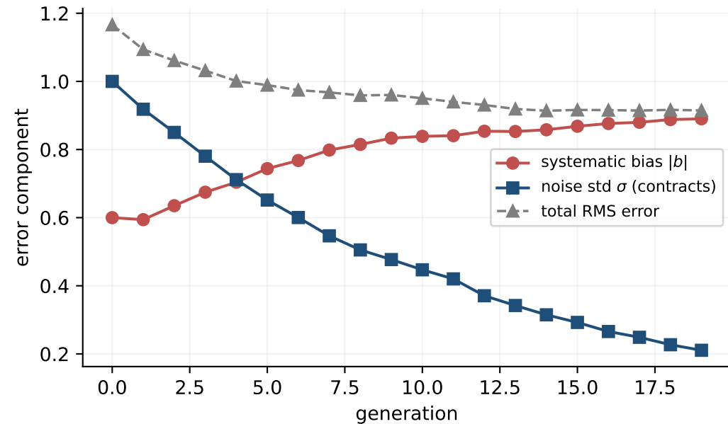
(a) single biased source: noise dies, bias survives
