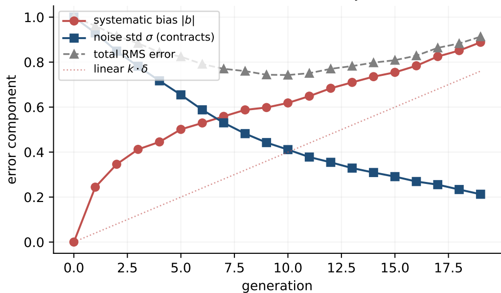
(b) per-generation artifact: bias accumulates ~linearly
