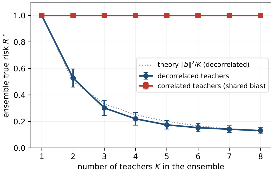
Decorrelated ensembling cancels inherited bias
