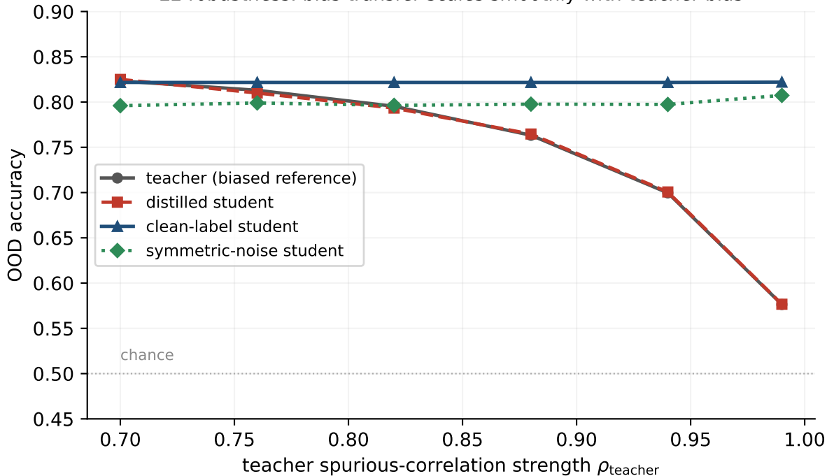
E2 robustness: bias transfer scales smoothly with teacher bias
