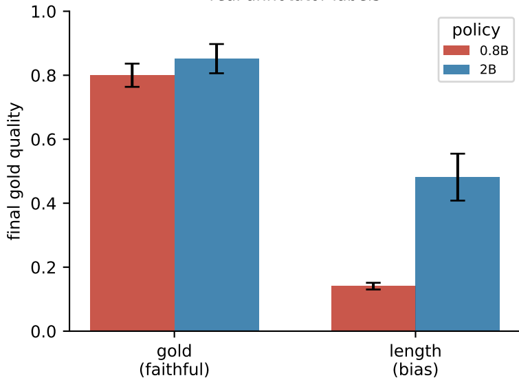
(a) Human feedback (RLHF) real annotator labels
