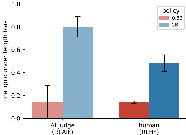
(b) Same bias, AI vs human 0.8B collapses in both
