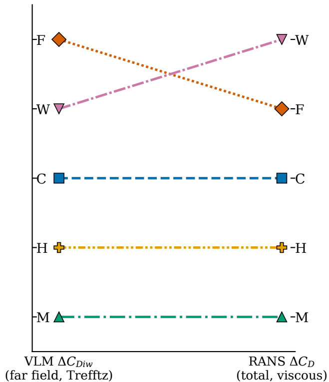
(b) far-field C_{Diw}
