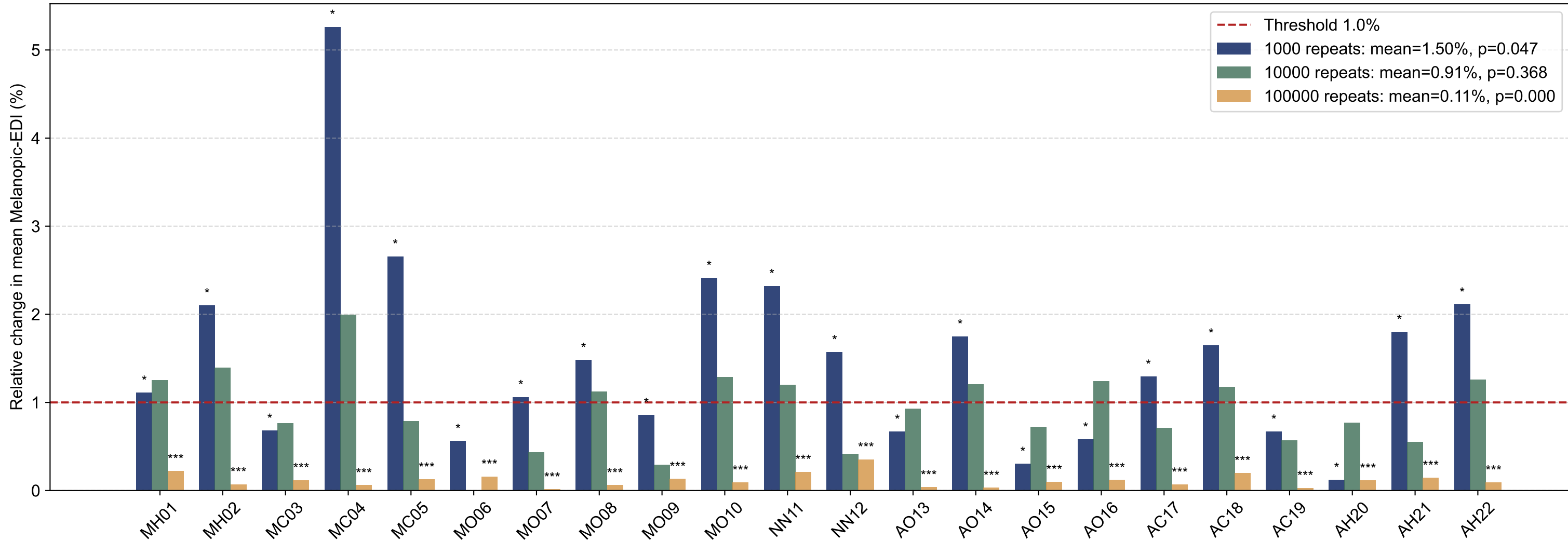
Monte Carlo stability per placeholder for multiple repeats
