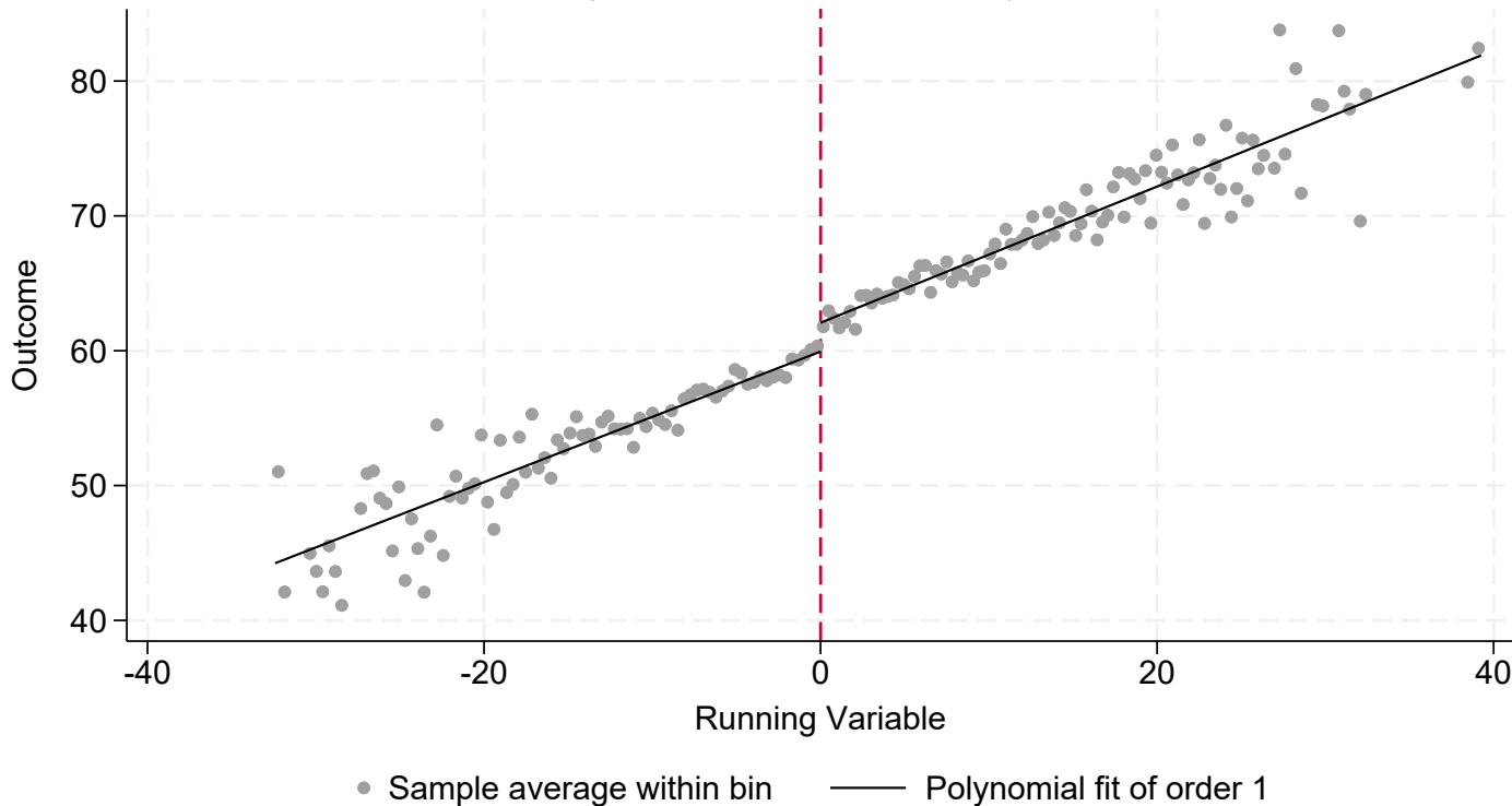
Regression Discontinuity Plot
