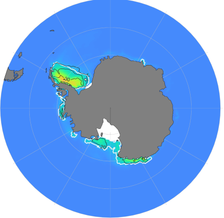
c2020d SIC Means & SD (JFM)
