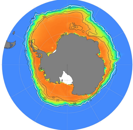
ct1950d SIC Means & SD (ASO)
