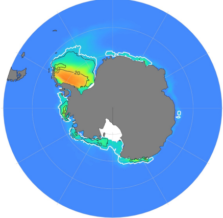
ct1950d SIC Means & SD (JFM)
