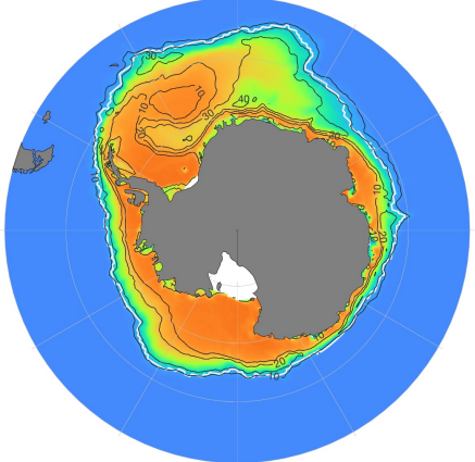
ssp585d SIC Means & SD (ASO)
