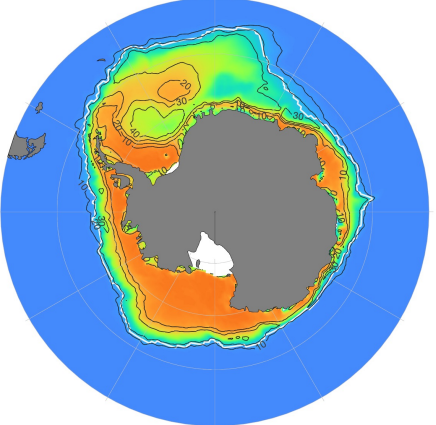
c2020d SIC Means & SD (ASO)
