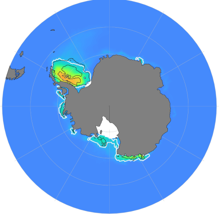
ssp585d SIC Means & SD (JFM)
