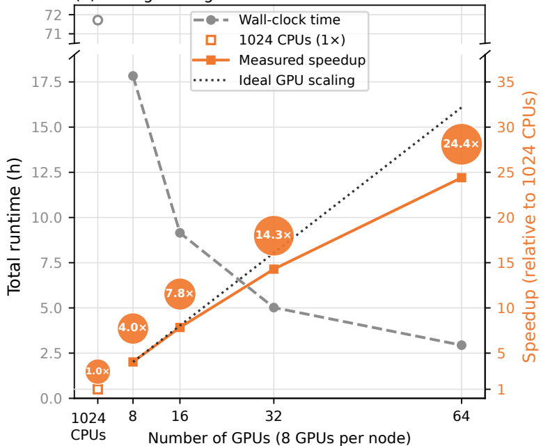
(a) Strong scaling
