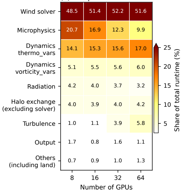
(b) Component time fraction
