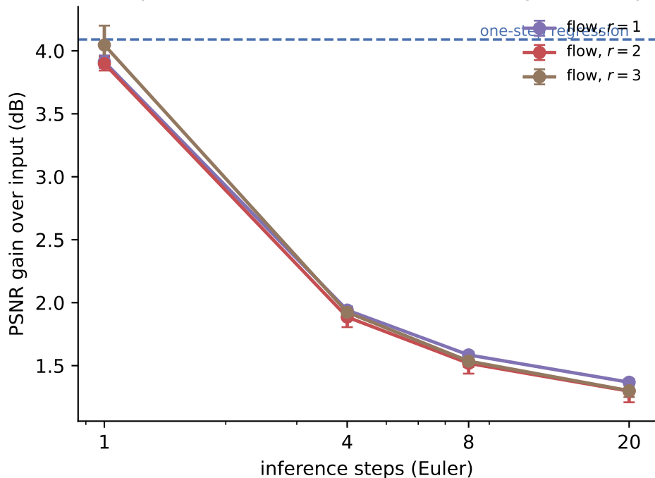
(b) Experiment: PSNR falls monotonically with steps
