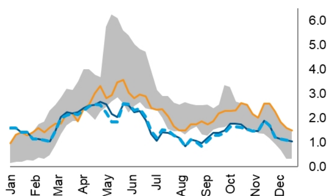
Fig 11 - Asia CDU T/A [MBD]
