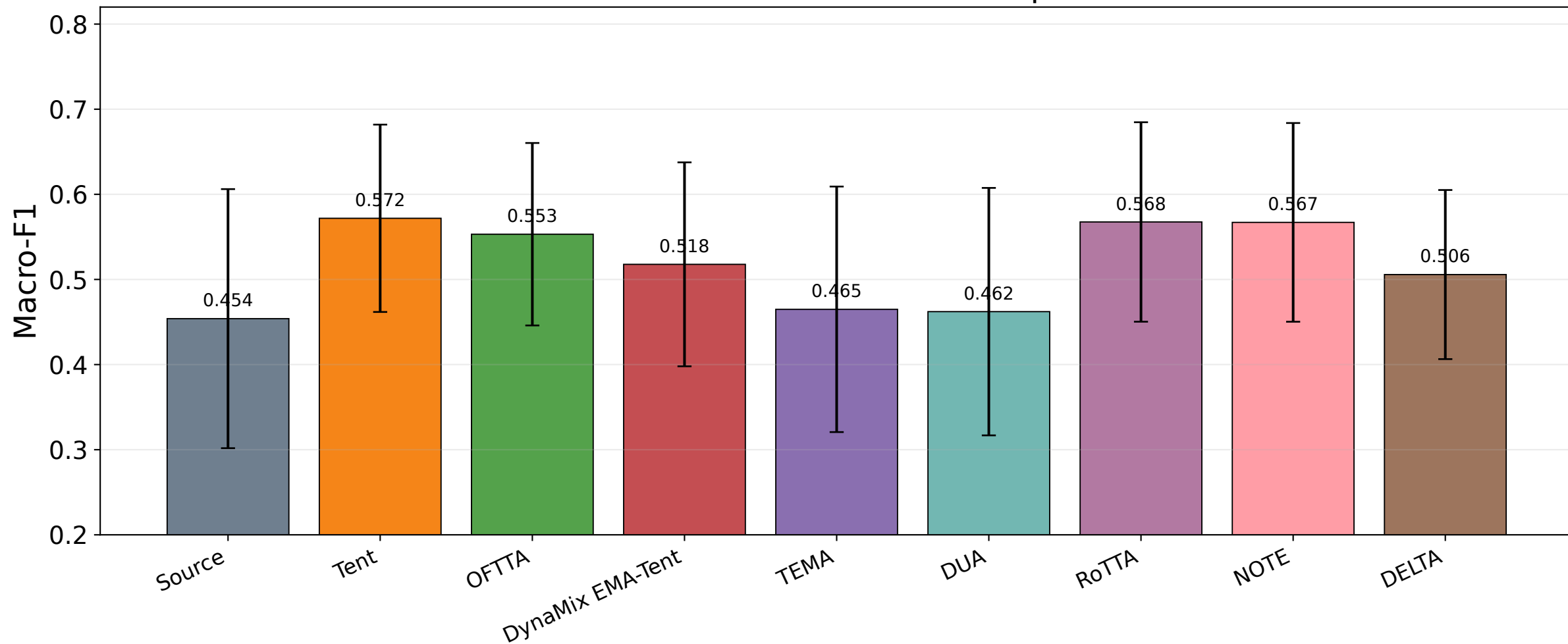
CASE valence: TTA method comparison
