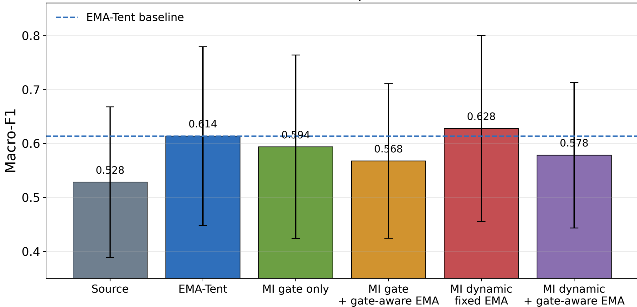
WESAD 3-class component ablation
