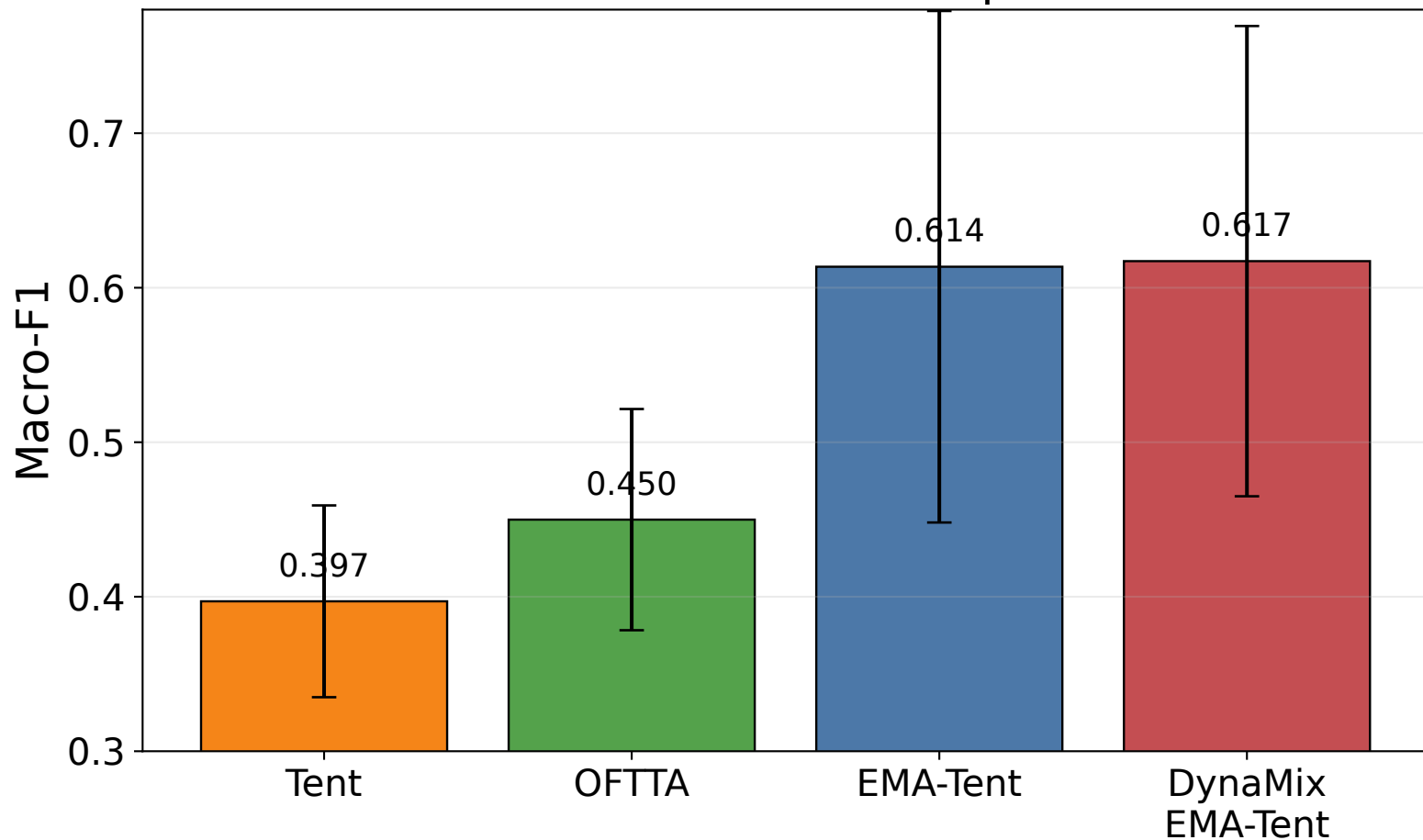
WESAD 3-class TTA comparison
