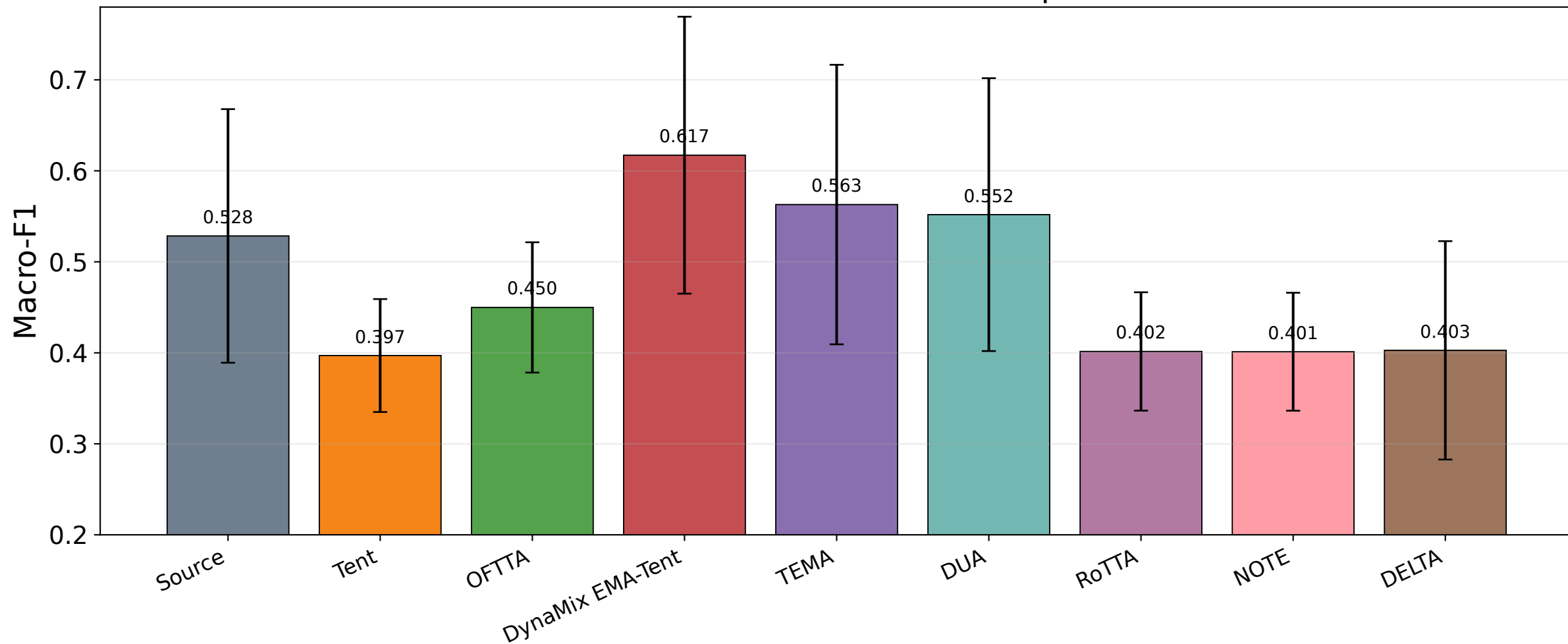
WESAD 3-class: TTA method comparison
