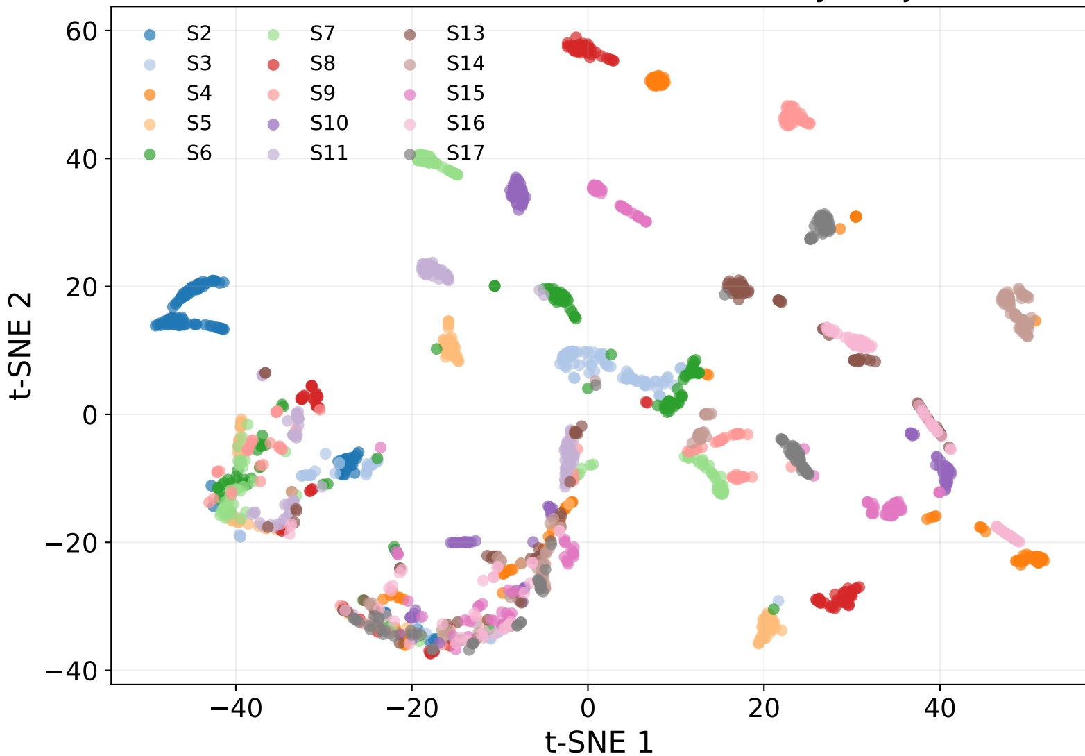
WESAD 1D-CNN features colored by subject
