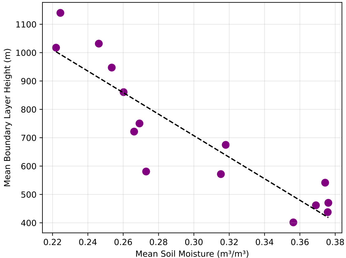
Soil Moisture vs BLH Correlation = -0.91
