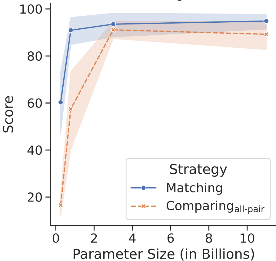
Recall@1
