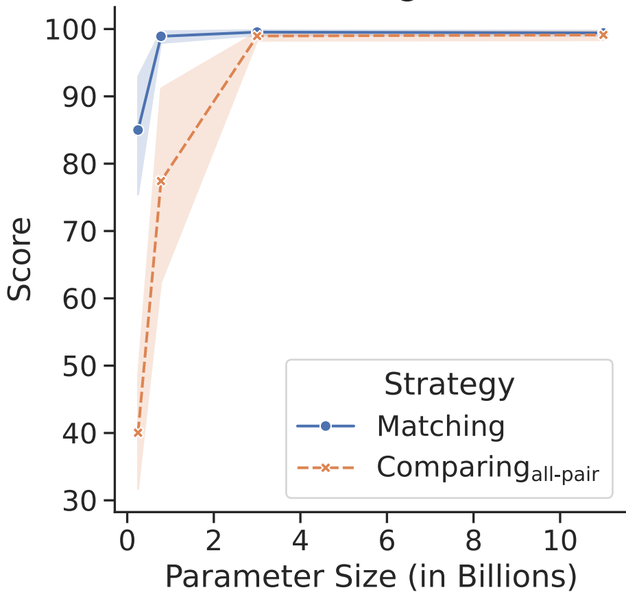
Recall@4
