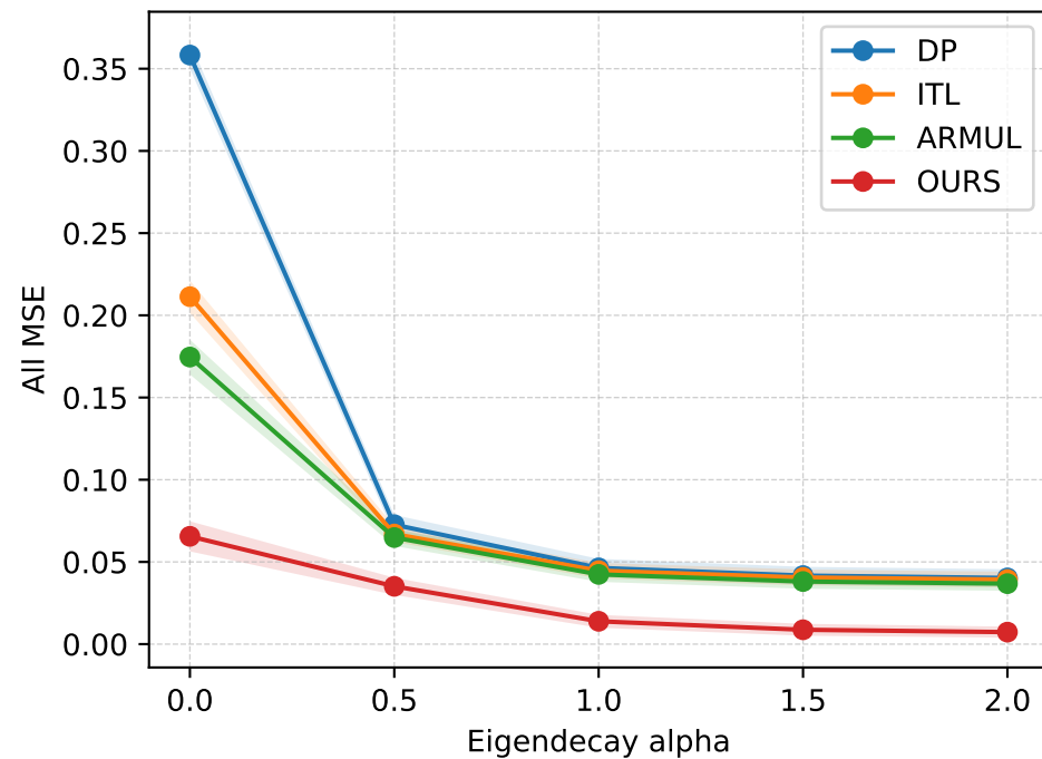
All tasks
