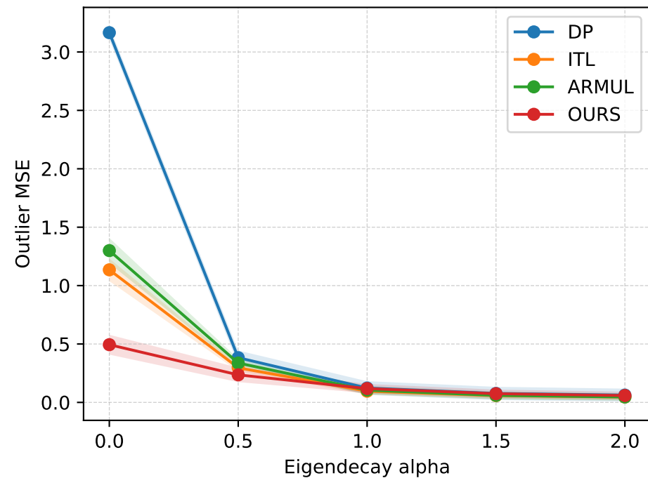
Outlier tasks
