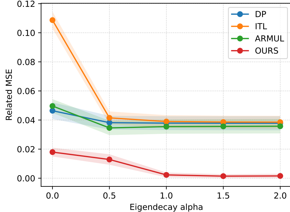
Related tasks
