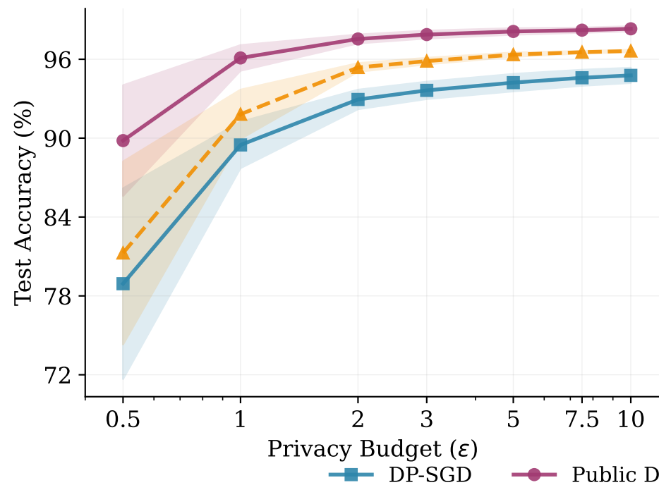
(a) StackOverflow
