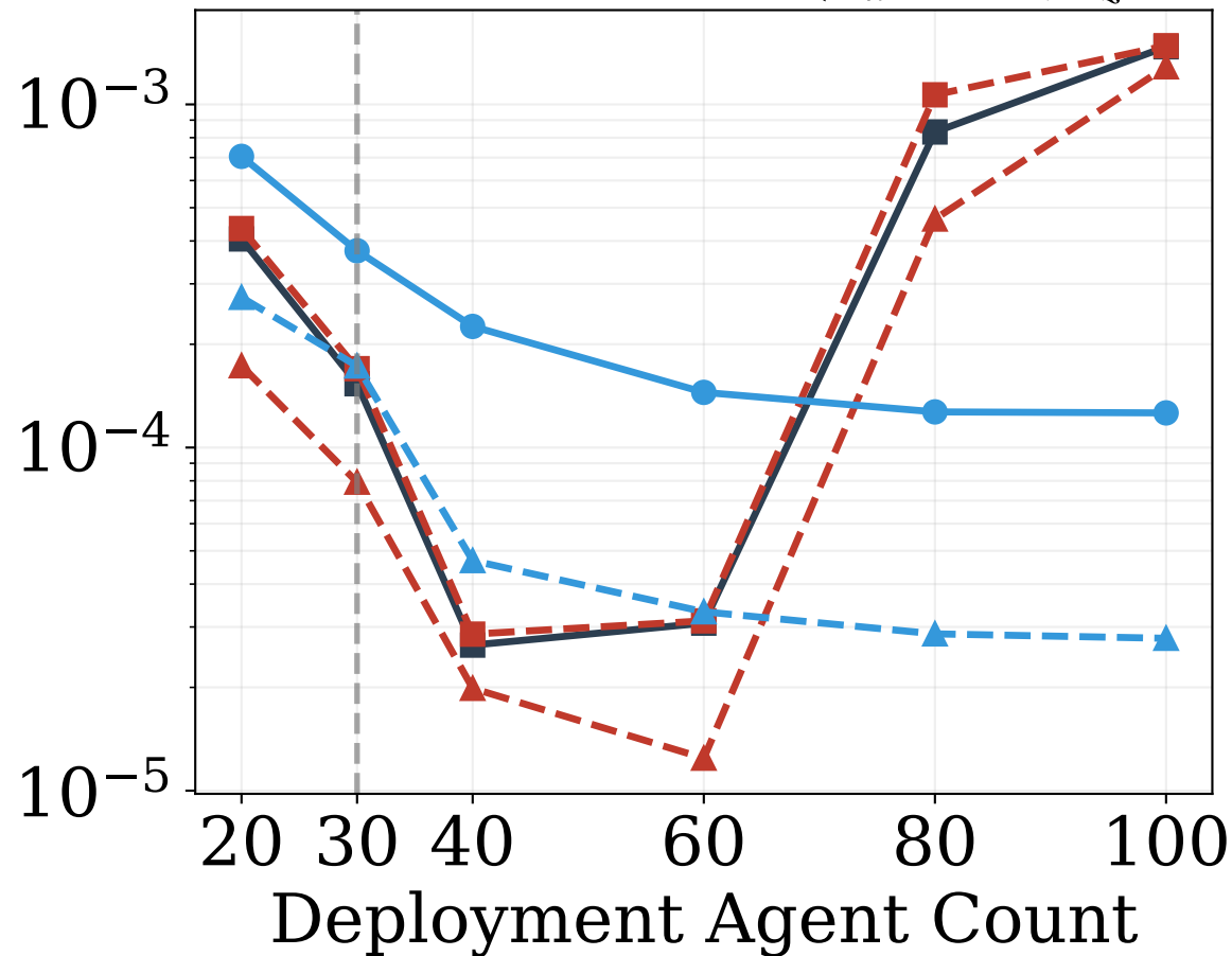
Mid Actuator Noise ( \sigma_u = 0.1, \sigma_z = 0.0 )
