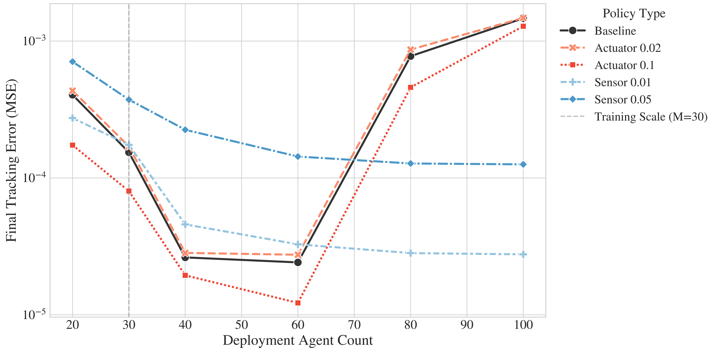
Robustness in Actuator Low Env ( \sigma_u = 0.02, \sigma_z = 0.0 )
